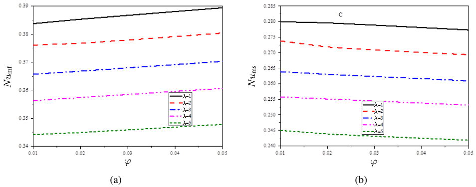
Figure 10. Variation of the average Nusselt number of fluid phase (a) and solid phase (b) for \text{Al}_2\text{O}_3\text{-Cu/water} hybrid nanofluid at Ha = 10, Q = 1, \varepsilon = 0.5, \delta = 0.5, H^* = 10 .
