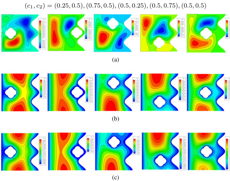
Figure 4. Contours of streamlines (a) isotherms of fluid phase (b) and isotherms of solid phase (c). Case C for \text{Al}_2\text{O}_3\text{-Cu/water} hybrid nanofluid at Ha = 10 , Q = 1 , \varepsilon = 0.5 , \delta = 0.5 , H^* = 10 .
