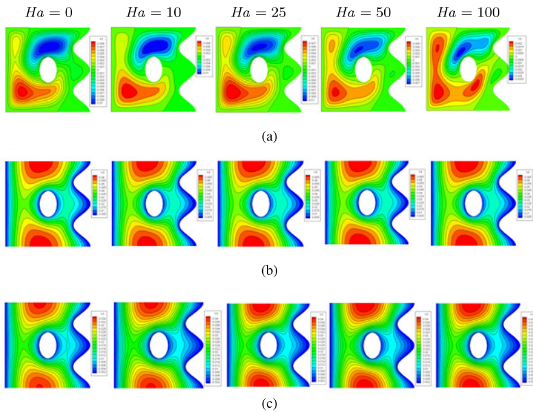
Figure 6. Contours of streamlines (a) isotherms of fluid phase (b) and isotherms of solid phase (c). Case B for \text{Al}_2\text{O}_3\text{-Cu/water} hybrid nanofluids at Q = 1 , \varepsilon = 0.5 , \varepsilon = 0.5 , H^* = 10 , Rd = 0.5 , \delta = 0.5 .
