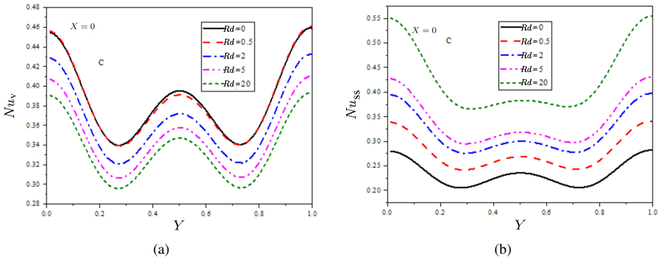
Figure 8. Profiles of the local Nusselt number of fluid phase (a), and solid phase (b) for \text{Al}_2\text{O}_3\text{-Cu/water} hybrid nanofluid at Ha = 10, Q = 1, \varepsilon = 0.5, \delta = 0.5, H^* = 10 .
