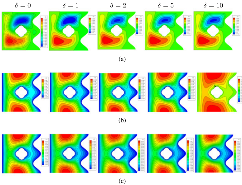
Figure 3. Contours of streamlines (a) isotherms of fluid phase (b) and isotherms of solid phase (c). Case C for \text{Al}_2\text{O}_3\text{-Cu/water} hybrid nanofluid at Ha = 10 , Q = 1 , \varepsilon = 0.5 , H^* = 10 , Rd = 0.5 .
