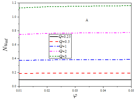
Figure 9. Variation of the average Nusselt number of fluid phase for \text{Al}_2\text{O}_3\text{-Cu/water} hybrid nanofluid at Ha = 10, \varepsilon = 0.5, H^* = 10, Rd = 0.5, \delta = 0.5 .
