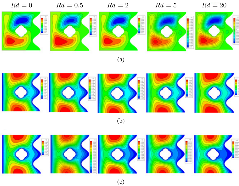
Figure 5. Contours of streamlines (a) isotherms of fluid phase (b) and isotherms of solid phase (c). Case C for \text{Al}_2\text{O}_3\text{-Cu/water} hybrid nanofluid at Ha = 10 , Q = 1 , \varepsilon = 0.5 , \delta = 0.5 , H^* = 10 .
