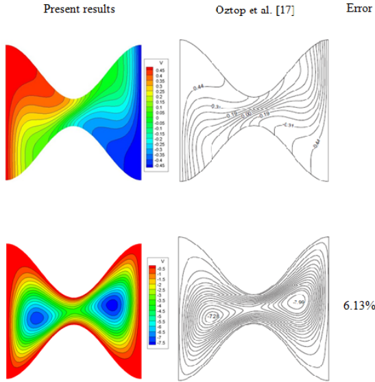
Figure 2. Validation test at Ra_E = Ra_l = 10^5 , a = 0.8 .
