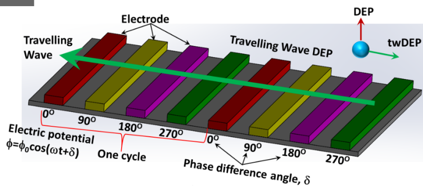
Figure 18. (a) Schematic representation of an array of microelectrodes for traveling wave DEP. Travelling waves are created by using phase difference of \pi/2 between the electrodes. Traveling wave DEP facilitates electrostatic force parallel to the direction of wave propagation in addition to the conventional vertical force. The phase difference creates spatial variation in the electric field which provides a movement of the suspended particles in the fluid media. Hence, it creates unidirectional flow of particles and an induced fluid motions in the microchannel.
