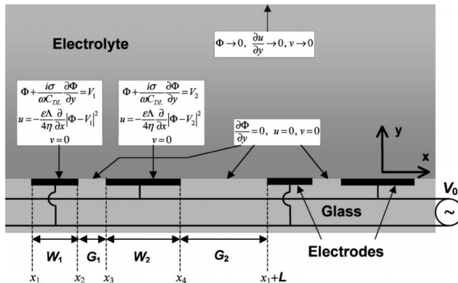
Figure 13. Schematic of the asymmetric electrode array for net fluid flow in a preferred direction. Boundary conditions for electric field and flow field are also presented for numerical simulation of ACEO. Reprinted this figure with permission from Ramos et al. [115]. Copyright (2003) by the American Physical Society.
