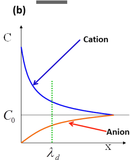
Figure 1. (a) Formation of an electric double layer next to a negatively charged surface. The Stern layer is also known as compact layer and it consists of inner and outer Helmholtz layer (not shown). The electrostatic action is very dominant in the Stern/compact layer. The diffuse layer is impacted by the Coulombic interaction and random thermal motion. (b) The qualitative plot of co-ion (anions) and counterions (cations) distribution in an electric double layer. The electrolyte is electroneutral in the bulk regime, where the concentrations of cations and anions are same.
