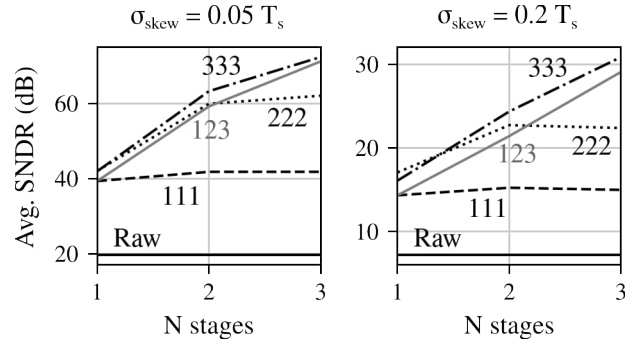
Fig. 5. Performance of different filter chain configurations in presence of normally distributed skew mismatch of deviation 0.05 T_s (left) and 0.2 T_s (right). Each point is an average of 100 trials with ideal 12-bit 8-channel TI-ADC sampling 770 MHz input signal at a rate of 2 GHz.
