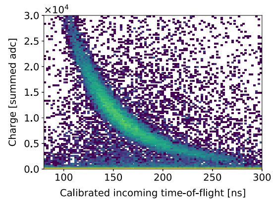
Fig. 9 Charge collected in the target PMT vs incoming time-of-flight for neutron-like events which were tagged in channel 5
