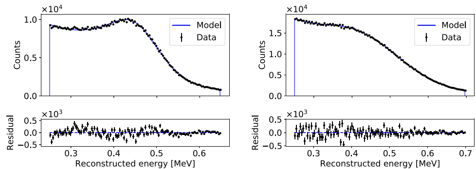
Fig. 4 Best fit charge models compared to LABPPO (left) and WbLS (right) calibration data using a 137 Cs source
