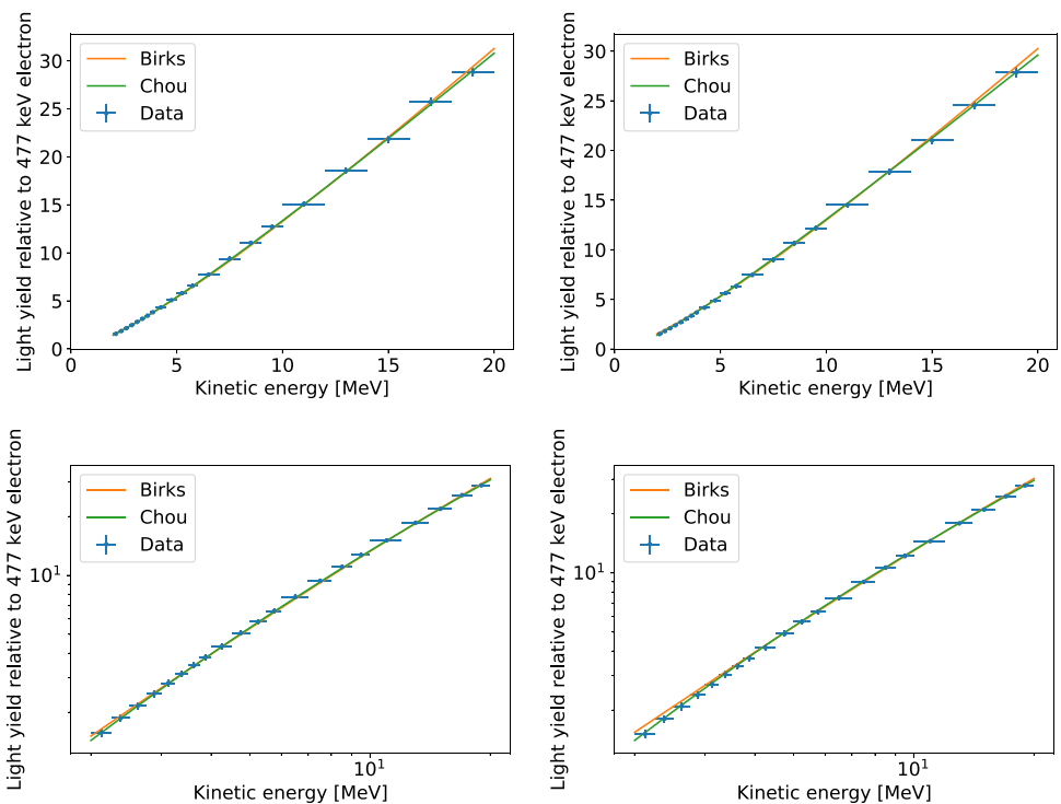
Fig. 13 Best-fit quenching models compared to the measured PLY for LABPPO (left) and WbLS (right), shown with both linear (top) and logarithmic (bottom) axes. The Birks model fails to reproduce the low-energy behavior of both materials, which is better modeled with the inclusion of the Chou bimolecular quenching term
