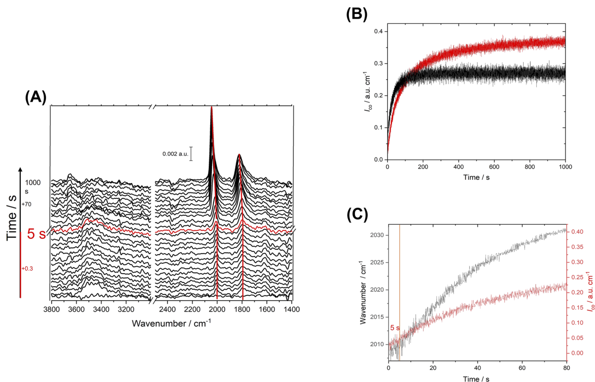
FIG. 2. (a) A typical time-resolved ATR-SEIRA spectral series showing the buildup of \text{CO}_{\text{ad}} on Pt in 0.1M \text{HClO}_4 containing 2 \times 10^{-3}\text{M} \text{HCOOH} , recorded after a potential step from 0.96 to 0.11 V vs RHE. Each spectrum consists of a single interferogram recorded with a spectral resolution of 16\text{ cm}^{-1} , resulting in a time interval between spectra of 0.15 s. The reference spectrum was taken at 0.96 V. Only selected spectra are shown. Between 0 and 5 s (red spectrum), a spectrum every 0.3 s is shown, whereas from that point onwards, a spectrum every 70 s is shown. (b) Time dependence of I_{\text{CO}_L} (red) and I_{\text{CO}_{B/M}} (black) during the whole experiment. (c) Time evolution of the stretching frequency of \text{CO}_L (black line) and of \text{CO}_B (red line) during the first 80 s.
