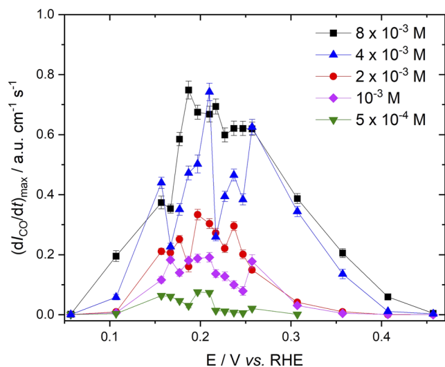
FIG. 4. Potential dependence of the rate of dehydration of HCOOH on Pt calculated by extrapolating to t = 0 the derivative of I_{\text{CO}_a} + I_{\text{CO}_b/\text{M}} at different concentrations of formic acid (ranging between 5 \times 10^{-4} and 8 \times 10^{-3} M, as indicated in the figure) in 0.1 M HClO 4 . Note that the error bars do not correspond to the standard deviation within a set of similar experiments but to the uncertainty in the rate of dehydration obtained by extrapolation at t = 0 , due to the noise present in the integrated intensity vs time curves.
