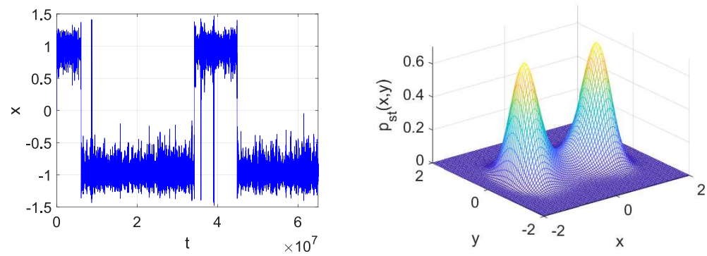
Figure 12. Same as Figure 11 for medium noise intensity.
