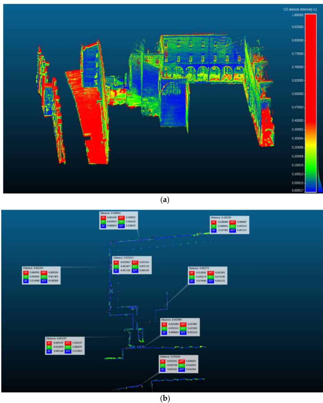
Figure 17. TF3: C2C comparison (a), and horizontal section with punctual measurements of the distance between the reference and the compared data (b).
