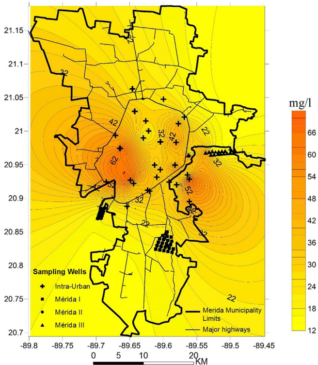
Fig. 6. Nitrate concentration (mg/l) in the study area (2012–2013).
