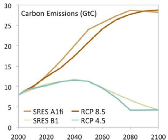
Figure i-3. Comparison of SRES and RCP Emission Scenarios (City of Cambridge, 2015)
