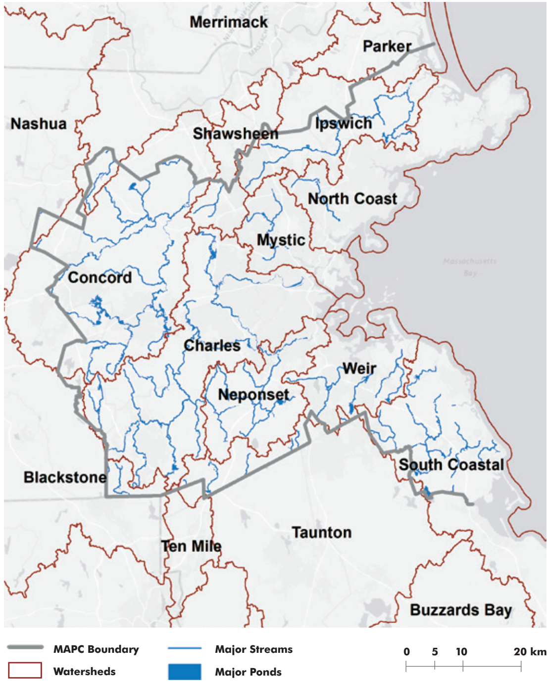
Figure 2.3 Major watersheds in the study area with major streams and lakes.
