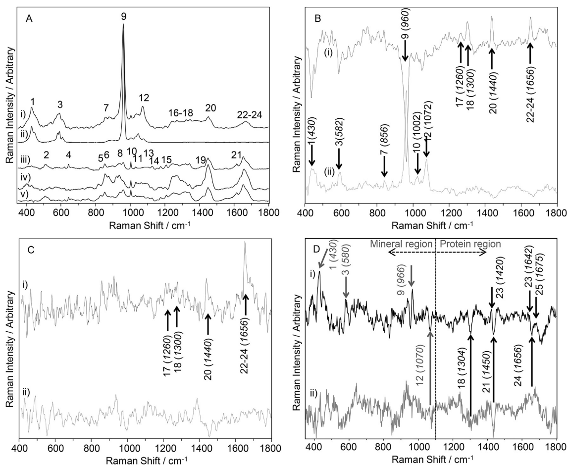
Fig. 2. Effect of ovariectomy model on the Raman signatures of bone and claw tissues. (A) Average normalised Raman spectra of Sprague-Dawley bone (i) and claw (iii) samples. The average spectra for the bone and claw models are compared to hydroxyapatite (ii), collagen (iv) and keratin (v). (B–C) Subtraction spectra for average (i) ovariectomy and (ii) sham ovariectomy minus baseline from bone (B) and claw (C) samples. Selected Raman bands are labeled against Table 2 with the corresponding wavelength in brackets. (D) The discriminant function for Sprague-Dawley bone (i) and claw (ii) samples as determined by the linear discriminant analysis (LDA) modelled on the respective ovariectomised (OVX) group against baseline group and projected onto the other treatment groups. The mineral peaks ( 350\text{--}1100\text{ cm}^{-1} ) are labeled in the bone spectra including peak number and wavenumber. While the corresponding protein peaks ( 1100\text{--}1800\text{ cm}^{-1} ) in the bone collagen and claw keratin are indicated including peak number and wavenumber.
