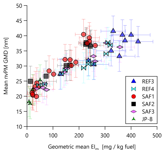
Figure 12. Scatterplot of the mean nvPM GMD within test points against geometric mean nvPM EI_m from Fig. 8a. The correlation with GMD and EI_m indicates that Fig. 9 implicitly represented different particle sizes.
