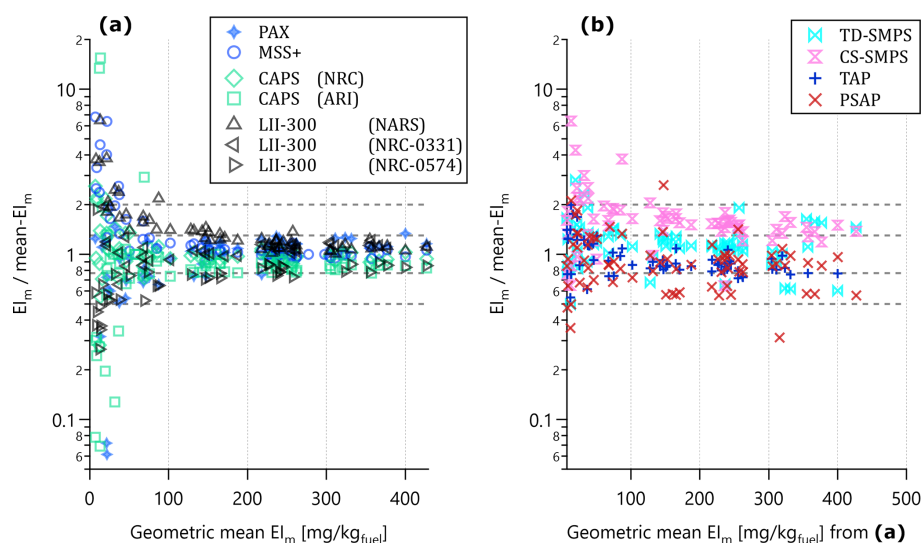
Figure 9. Ratio plots corresponding to Fig. 8. The inner and outer horizontal lines show ratios of 2, 2^{-1} , 1.3, 1.3^{-1} , and 1.0. Agreement between the instruments is poorer at EI_m < 100 mg per kg fuel, which corresponds to an approximate concentration of 10 \mu\text{g m}^{-3} (the exact conversion factor varies with \text{CO}_2 concentration and fuel properties) and is close to the limit of detection for most instruments.
