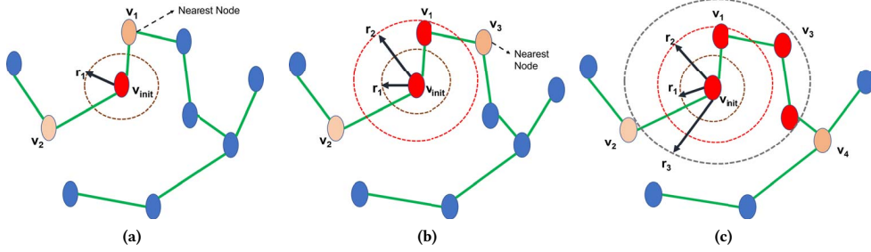
Figure 2: (a) A region around the initial node. (b) Increased radius for the region based on the nearest segment whose one connecting end is inside the previous region. (c) A region where the volume is greater than cut.
