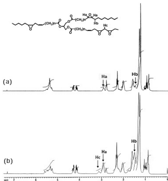
Figure 2. ^1\text{H} NMR spectra of (a) ELO_2 epoxidized 20%, and (b) ELO_6 epoxidized 54%.
