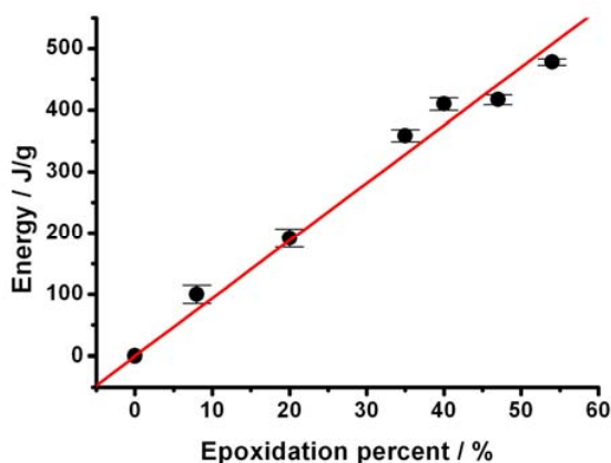
Figure 5. Curve showing a linear correlation between calculated epoxidized degree and epoxy aperture energy.
