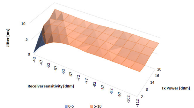
Fig. 8. Jitter vs Tx power and receiver sensitivity for scenario 1.
