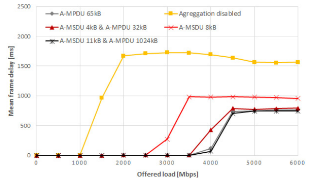
Fig. 12. Frame delay vs offered load for scenario 2.
