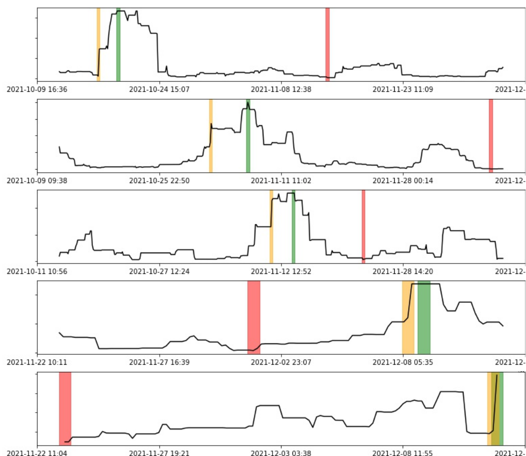
Figure 3. Normalised periodicity intensity for a sample of five student participants. Frequency is 24 hours, window size is 7 days and window shift or stride is 3 hours. Y-axis values have been normalised to the range 0 to 1.
