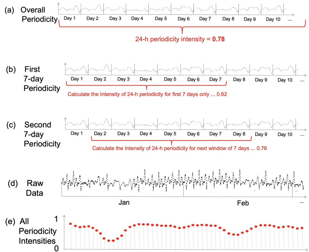
Figure 1. Schematic demonstrating the calculation of periodicity intensity throughout a time series using time-lagged overlapping windows.
