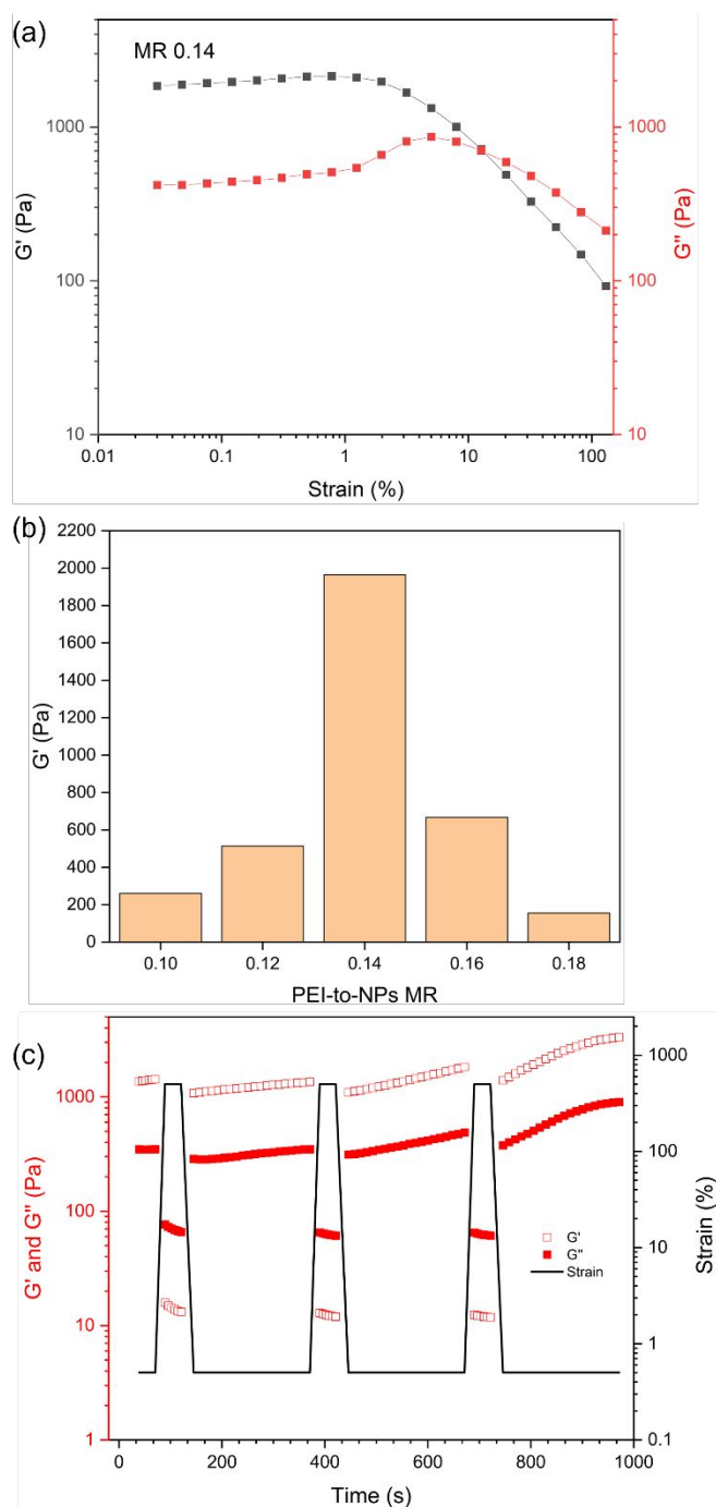
Figure 4. Rheology characterisation of PNCC hydrogels containing bPEI and PISA derived nanoparticles; (a) Strain-dependent ( \omega = 10 \text{ rad s}^{-1} , 25^\circ \text{C} ) oscillatory shear rheology of bPEI/ S_{68}\text{-P}(\text{B}_{0.6}\text{-A}_{0.4})_{300} _MR0.14 hydrogel (20% w/w); (b) gel strength of bPEI/ S_{68}\text{-P}(\text{B}_{0.6}\text{-A}_{0.4})_{300} mixtures (20% w/w) at different bPEI-to-NPs mass ratio (MR = 0.10, 0.12, 0.14, 0.16, 0.18); (c) High (500%) and low (0.5%) strain steps for bPEI/ S_{68}\text{-P}(\text{B}_{0.6}\text{-A}_{0.4})_{300} _MR0.14 hydrogel (20% w/w) over three cycles ( \omega = 10 \text{ rad s}^{-1} , 25^\circ \text{C} ).
