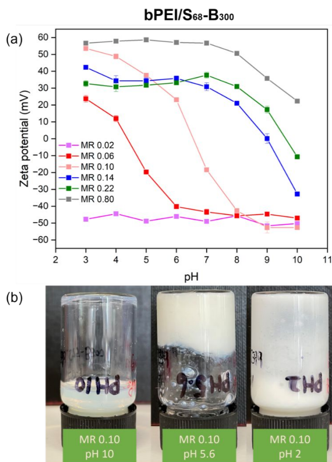
Figure 2. (a) Zeta potential vs. pH curves for dilute aqueous dispersions containing mixture of bPEI/S 68 -B 300 mixtures with various bPEI-to-NPs MRs; (b) Digital image of fluids and precipitates for bPEI/S 68 -B 300 mixtures at MR 0.10 (20% w/w) obtained at different pH values.
