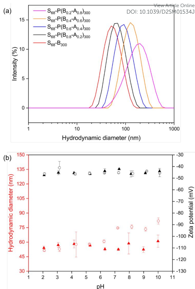
Figure 1. S_{68} -P(B m -A 1-m ) 300 diblock copolymer nanoparticles prepared at 20 % w/w solids via RAFT-mediated statistical copolymerisation of BzMA and MAA in water at pH 2. (a) DLS intensity-average size distributions of S_{68} -P(B m -A 1-m ) 300 ( m = 0.2, 0.4, 0.6, 0.8, 1.0 ) dispersions at pH 10; (b) dynamic light scattering and aqueous electrophoresis data as a function of pH obtained for S_{68} -B 300 (triangles) and S_{68} -P(B 0.6 -A 0.4 ) 300 (circles) diblock copolymer nanoparticles. Measurements were conducted at a copolymer concentration of approximately 0.1 % w/w in the presence of 1 mM KCl as a background electrolyte.
