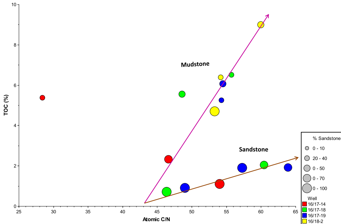
Figure 9. Relationship between TOC and C/N ratio showing different trends for sandstone-dominated and mudstone-dominated samples for core plugs from four Quadrant 16 wells, UK. Note the one anomalous point with high TOC and a low C/N atomic ratio.
