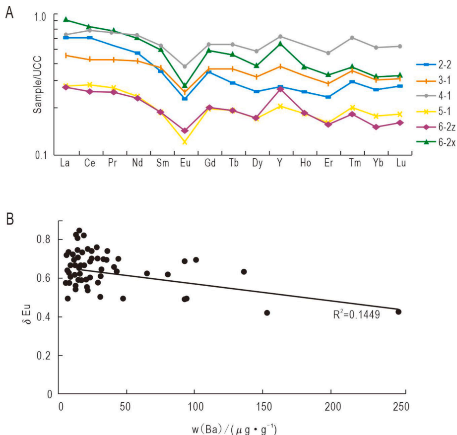
Fig. 5. Distribution patterns of REY in the samples. (A) REY are normalized by Upper Continental Crust (UCC) (Taylor and McLennan, 1985). (B) Diagram of the relationship between \delta Eu and \omega(Ba) of samples.
