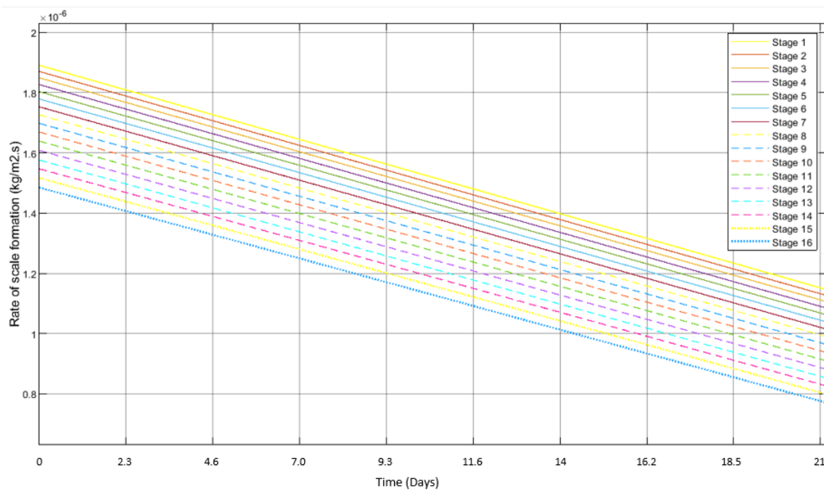
Figure 5. Profiles of rates of scale formation amongst the stages in MSF-OT as derived from the Simulink model.
