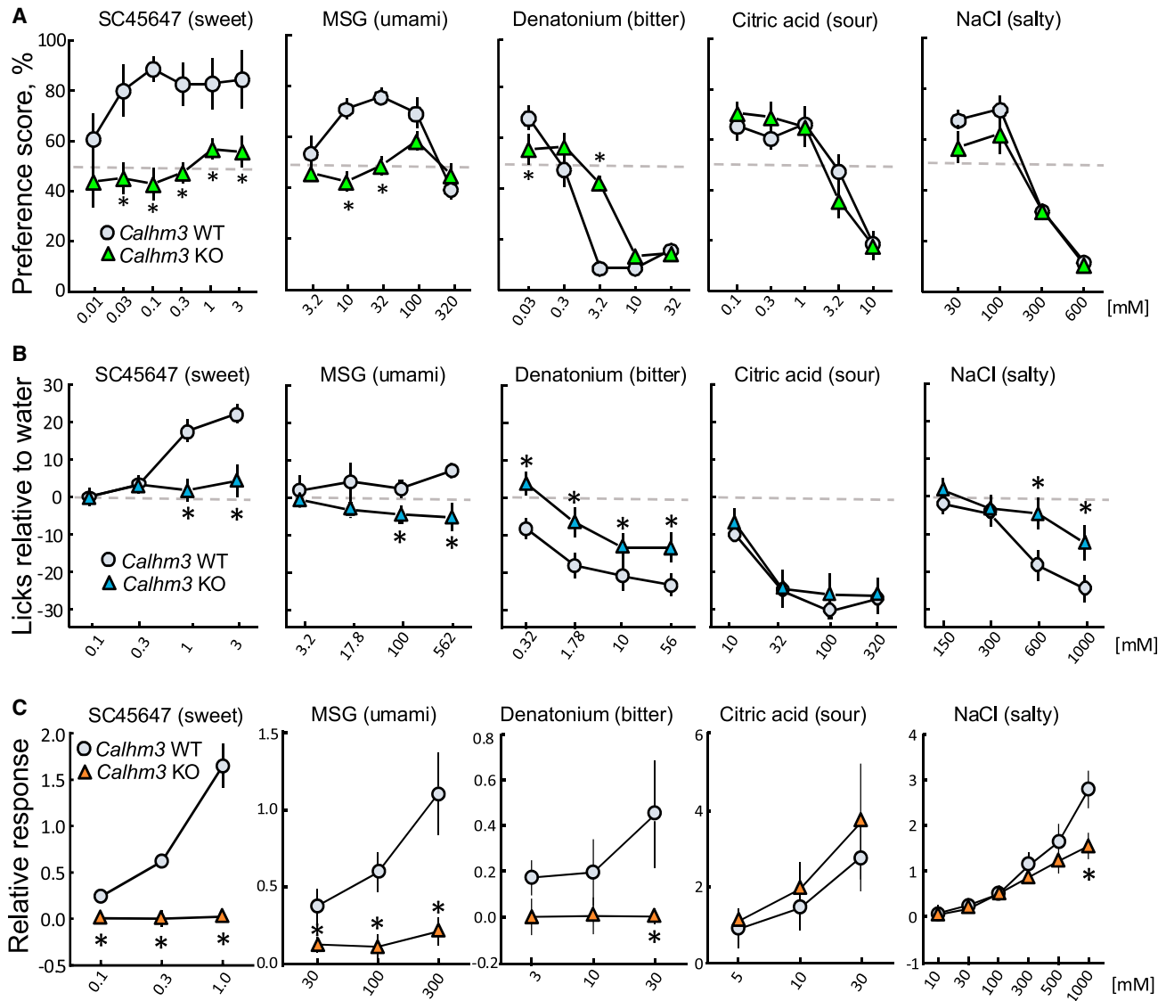
Figure 8. CALHM3 Is Essential for GPCR-Mediated Taste Perception
