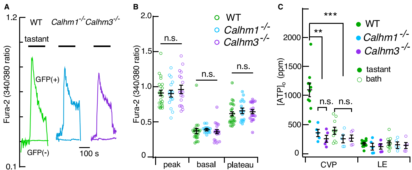
Figure 7. Type II TBC [Ca^{2+}]_i Signaling Is Normal Whereas ATP Release Is Abolished in Calhm1^{-/-} and Calhm3^{-/-} Mice
