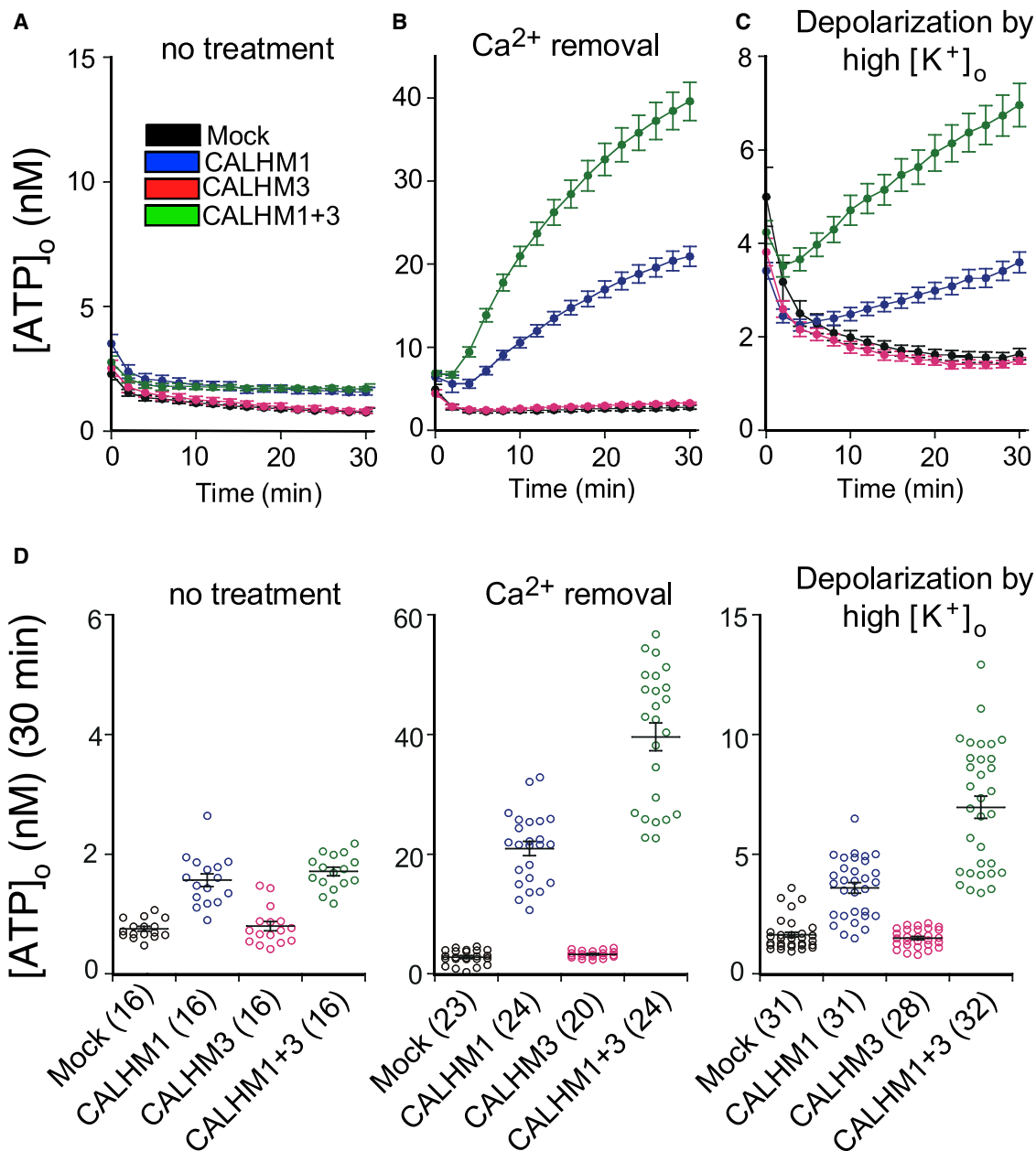
Figure 2. CALHM3 Accelerates CALHM1-Mediated ATP Release
