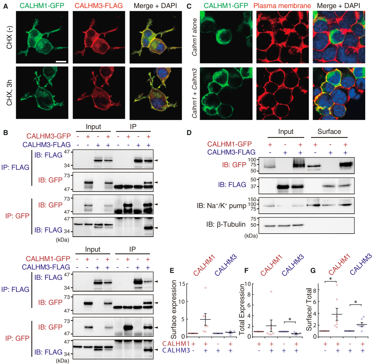
Figure 3. CALHM3 Co-localizes and Interacts with CALHM1
