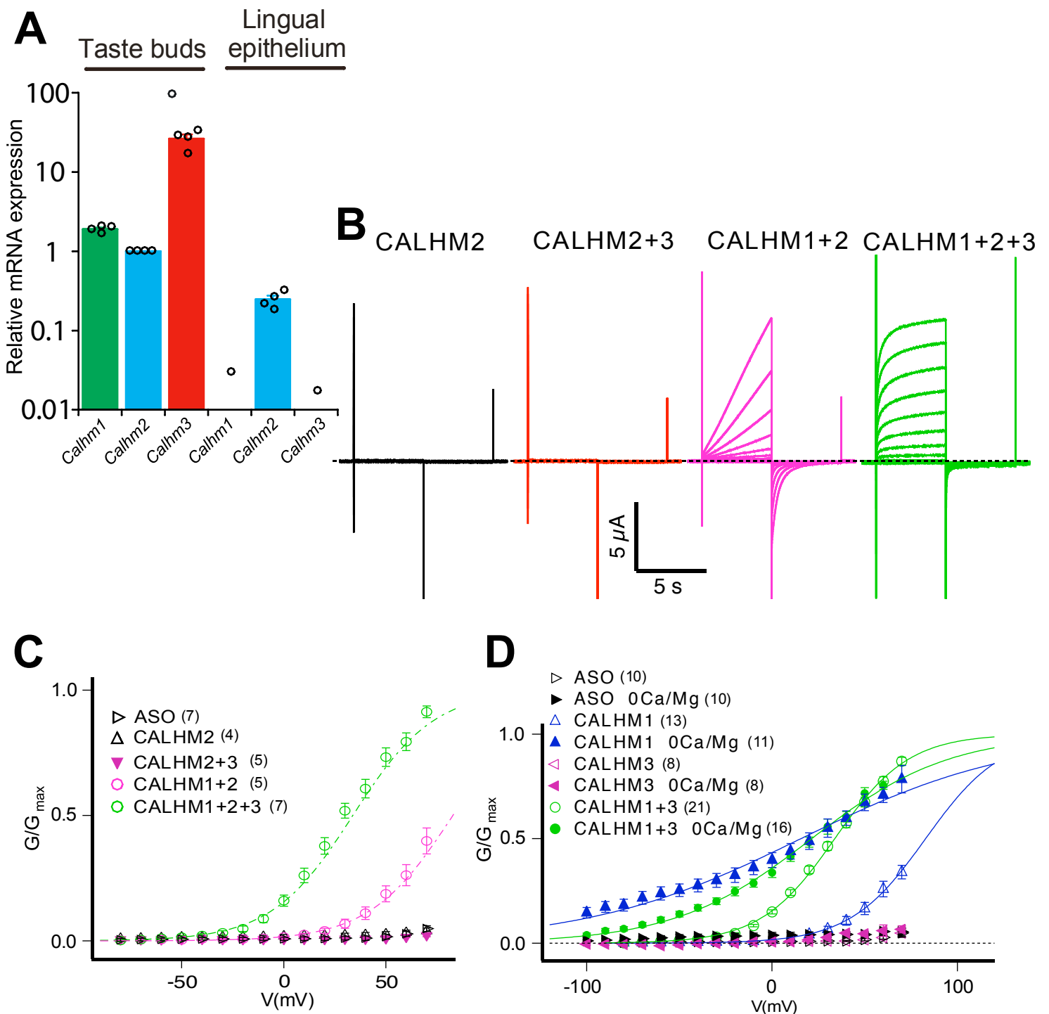
Figure S1. Lack of CALHM2 function in Xenopus oocytes, related to Figure 1
