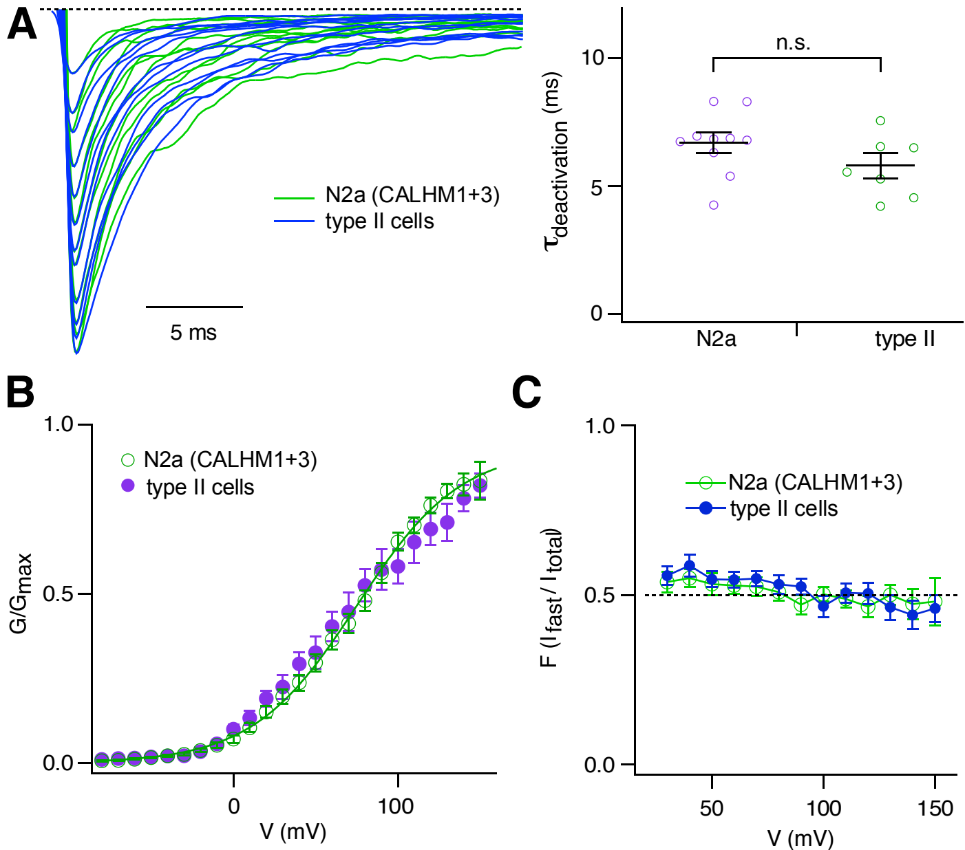
Figure S6. Similar Voltage-dependent Gating Properties of ATP-release Channel Currents in Type II Cells and in N2a Cells Co-expressing CALHM1 and CALHM3, related to Figure 5
