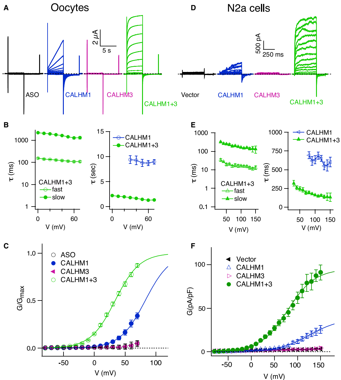
Figure 1. CALHM3 Enhances Voltage-Dependent Gating of CALHM1 Channels
