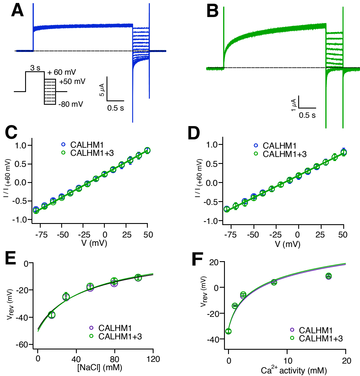
Figure S2. Co-expressing CALHM3 with CALHM1 Does Not Alter Relative Ionic Permeabilities, related to Figures 1 and 2
