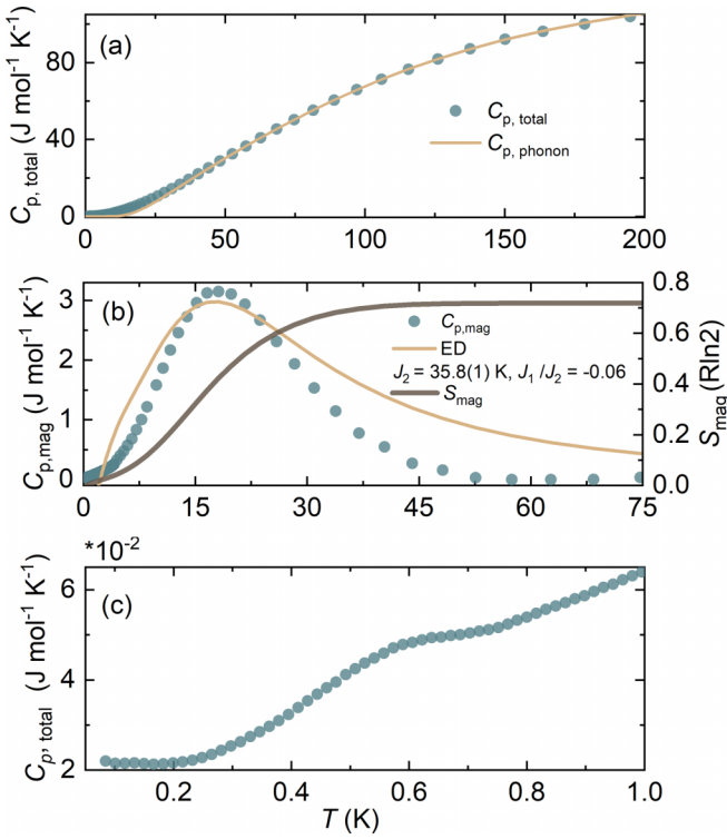
FIG. 4. (a) Temperature dependence of the zero-field total heat-capacity fit to a Debye-Einstein model to approximate the phonon contribution to the specific heat, C_{p,\text{phonon}} , yielding \theta_D \simeq 550 K, f_D \simeq 0.58 , \theta_{E_1} \simeq 90 K, f_{E_1} = 0.11 , \theta_{E_2} \simeq 115 K, f_{E_2} = 0.13 , \theta_{E_3} \simeq 460 K, and f_{E_3} = 0.18 . By subtracting C_{p,\text{phonon}} from the total heat capacity (b), (left), the resulting magnetic specific heat, C_{p,\text{mag}} , reveals a broad feature centered about 18 K and that can be described by the S = \frac{1}{2} Heisenberg frustrated chain model with an intrachain exchange parameter, J_2 = 35.8(1) K, and an interchain exchange parameter, J_1/J_2 = -0.06 . This feature is also associated with (b), (right) magnetic entropy release. (c) A broad feature, centered about T_N = 0.54 K, is observed in C_{p,\text{total}} .
