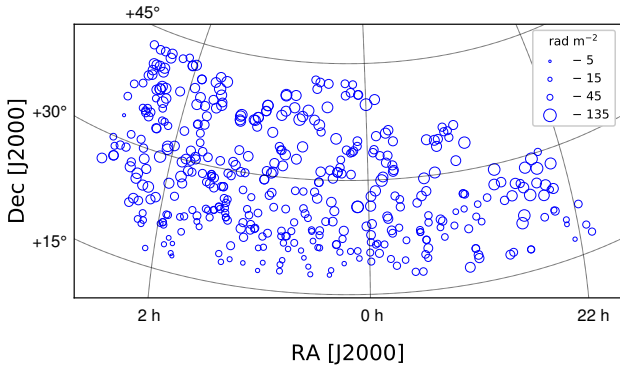
Figure 4. In a similar manner to Fig. 3, this shows the sky distribution of the polarized sources across the LoTSS-DR2 0 hr field. There are 422 sources in the 0 hr field, which corresponds to an areal number density of 0.29 \text{ deg}^{-2} .
