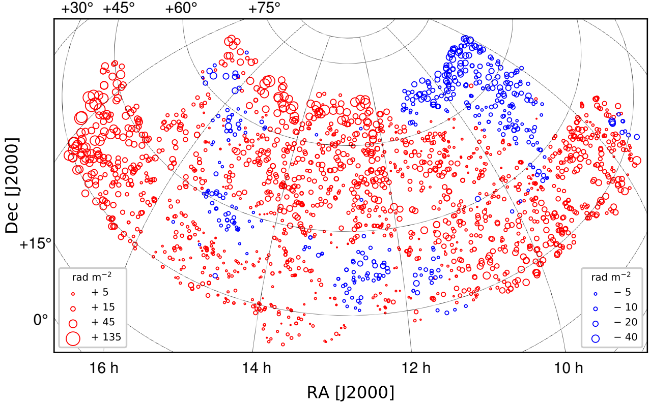
Figure 3. Sky distribution of the polarized sources across the LoTSS-DR2 13 hr field, in equatorial coordinates and with an orthographic projection. The red/blue coloured circles correspond to positive/negative RM values, and the size of the circles are proportional to the magnitude of the RM (as quantified in the figure legends). There are 2,039 sources in the 13 hr field, which corresponds to an areal number density of 0.48 \text{ deg}^{-2} .
