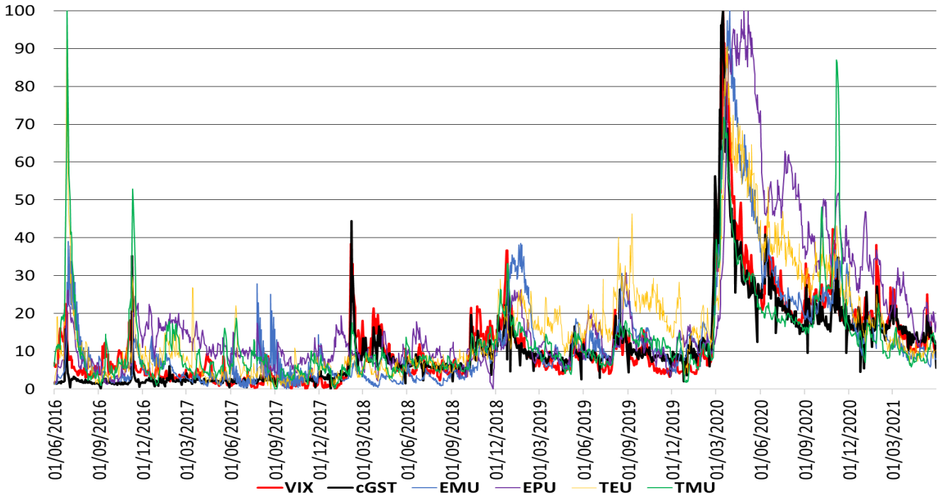
Figure 2: cGST_t in levels with uncertainty measures
