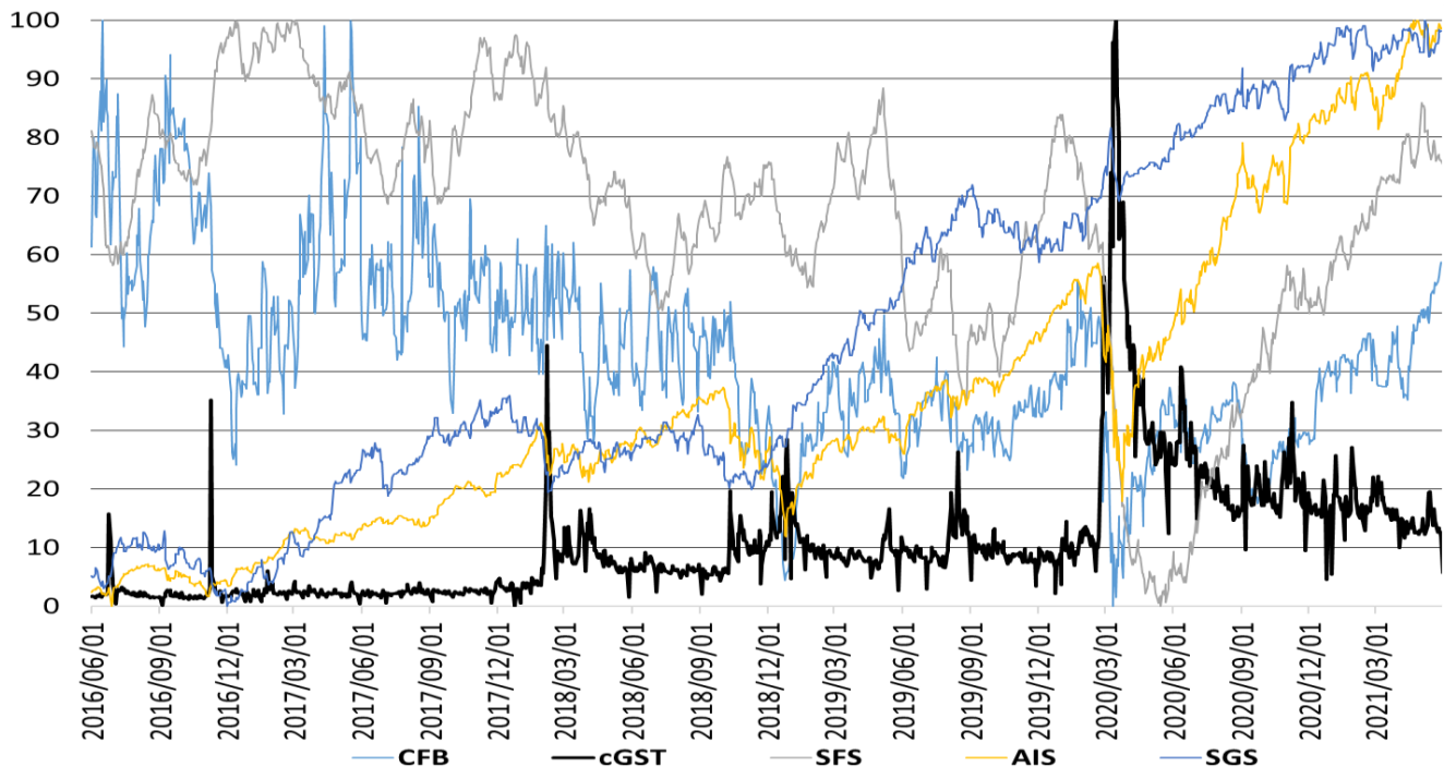
Figure 3: cGST_t in levels with sentiment measures
