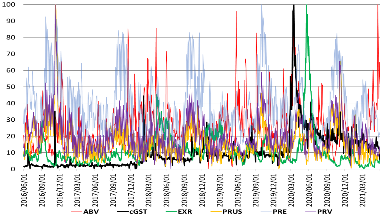
Figure 4: cGST_t in levels with attention measures
