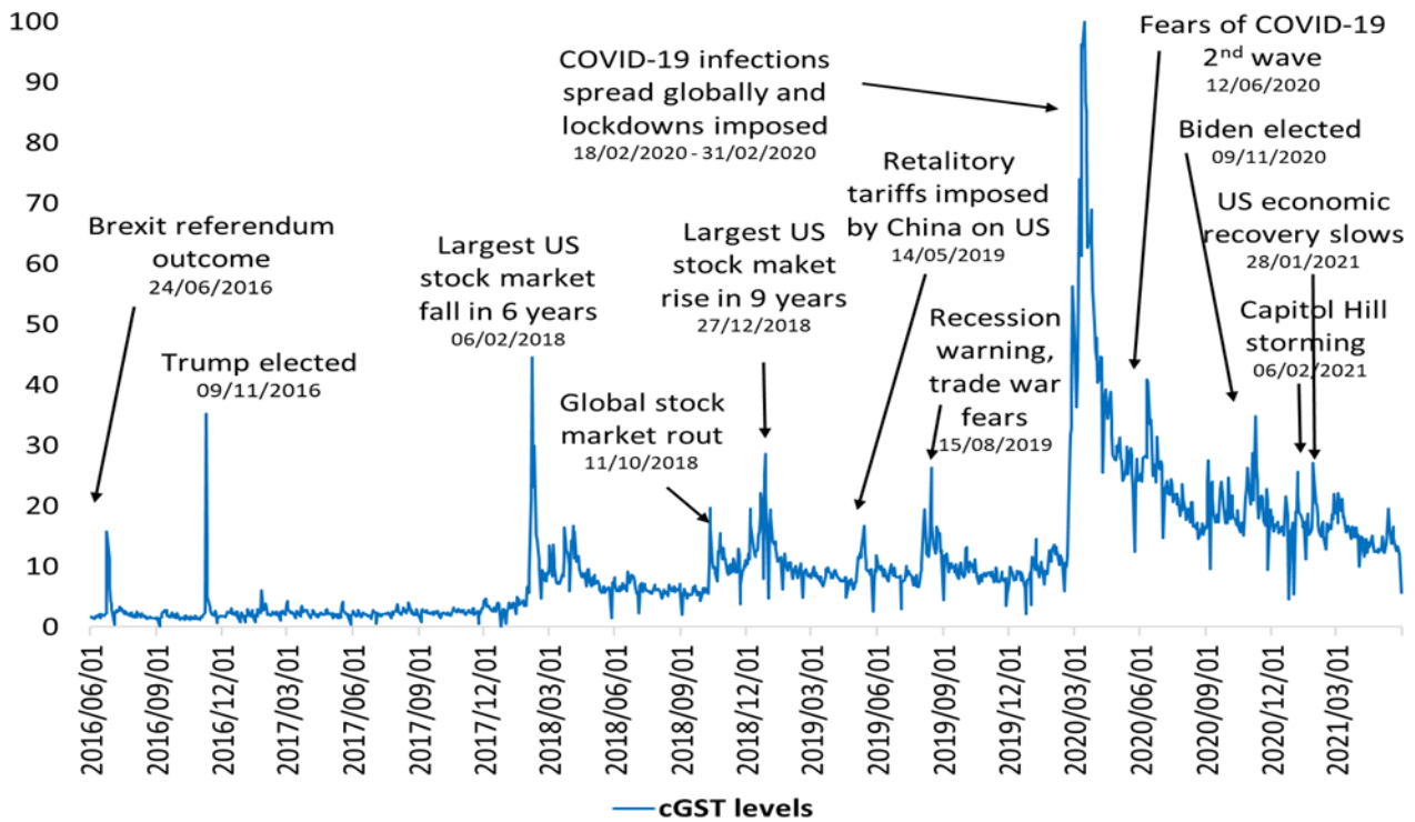
Figure 1: cGST_t in levels with significant events
