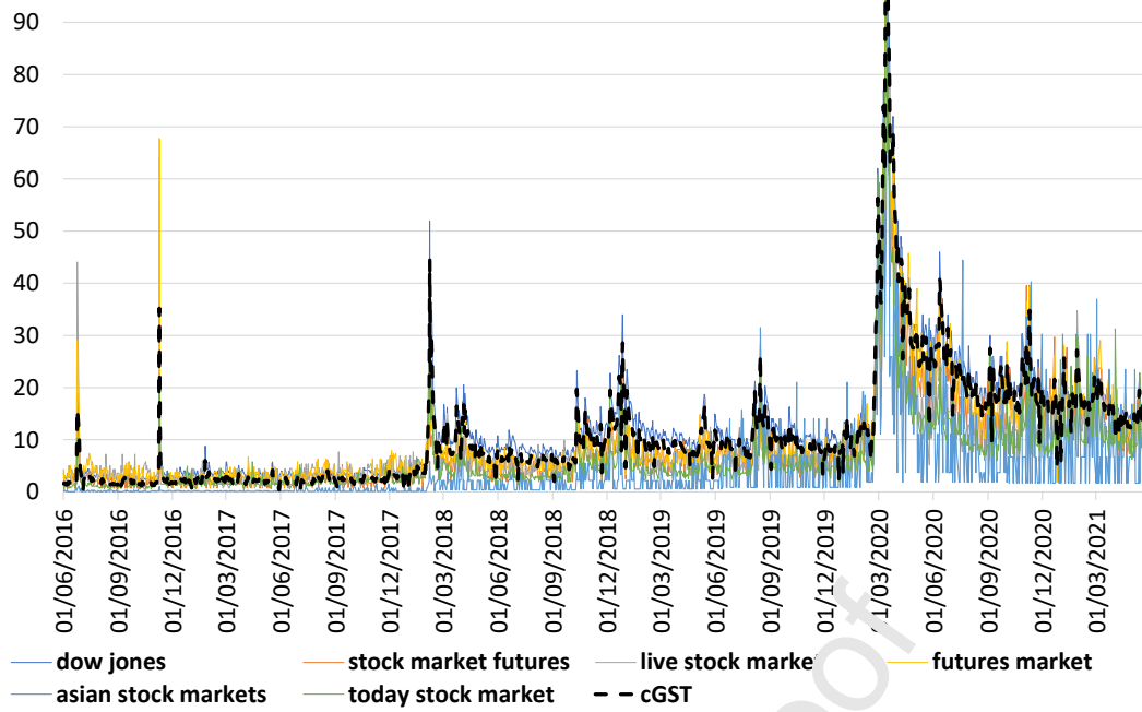
Figure A2: cGST_t and constituent terms
