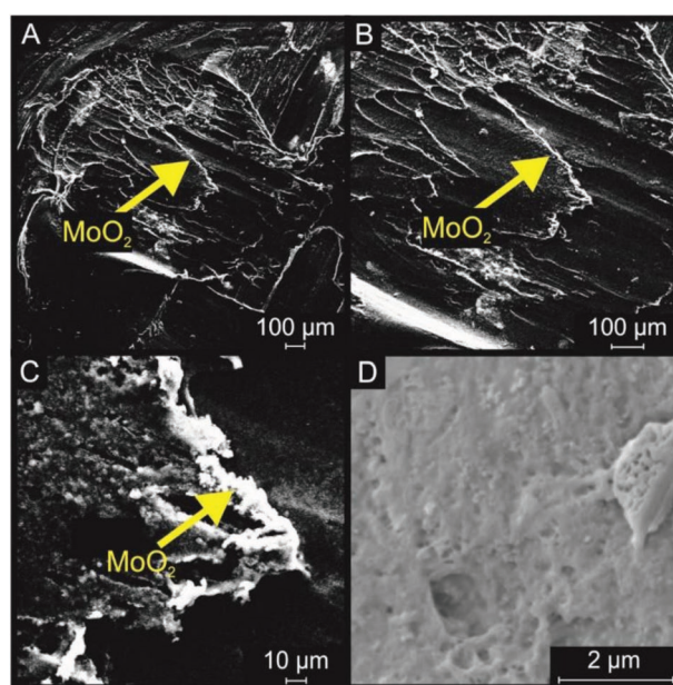
Figure 4. SEMs of A,B,C) MoO 2 -G/AME and D) G/AME. Electrochemical decoration parameters: -1.4 V, 600 s.
