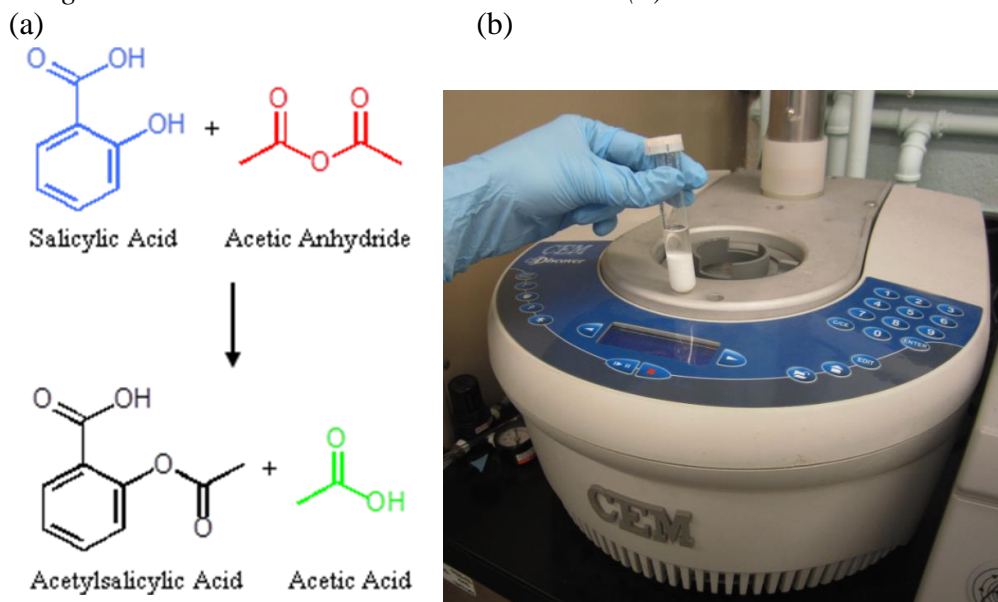
Figure 2. Aspirin Synthesis. The reaction of salicylic acid and acetic anhydride yielding acetylsalicylic acid (aspirin) and acetic acid (a) can be prepared using a CEM DISCOVER industrial microwave (b)
