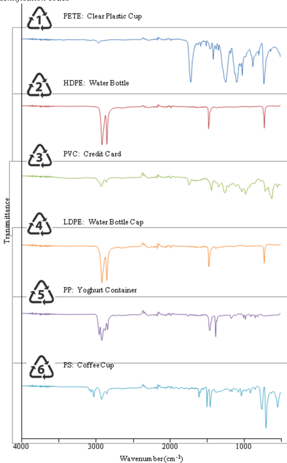
Figure 5. ATR-IR Spectra. Household polymers with different resin identification codes
