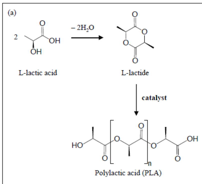
Figure 6. Poly(lactide) (PLA) Synthesis. (a) PLA production from L-lactic acid or lactide. (b) ^1\text{H} NMR spectra showing the methine proton in the lactide monomer (top panel) and in PLA (bottom panel) dissolved in \text{CDCl}_3 (c) ATR-IR spectra of L-lactide and PLA
