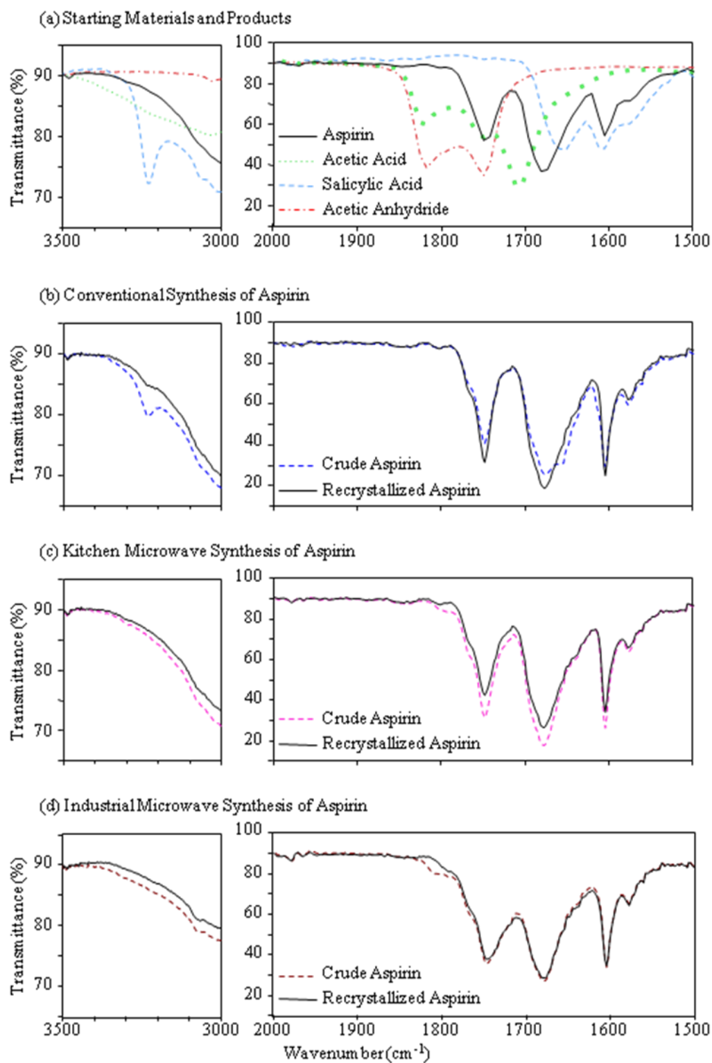
Figure 3. Aspirin Synthesis. A comparison of the ATR-IR spectra of (a) the starting materials and pure products, and the crude and recrystallized aspirin products obtained by (b) conventional, (c) kitchen microwave and (d) industrial microwave syntheses
