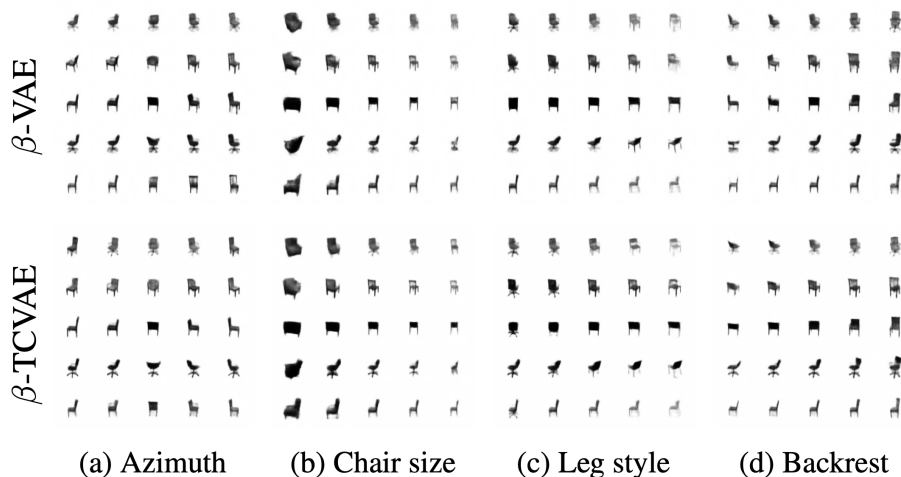
Figure 3: Latent traversal of dimensions in representation spaces disentangled using \beta -VAE (top rows) (Higgins et al., 2017) and \beta -TCVAE (bottom rows) (R. T. Q. Chen et al., 2018). Respective traversals along dimensions in the representation space exhibit changes in the observable factors of (a) Azimuth (b) Chair size (c) Leg style and (d) Backrest.
