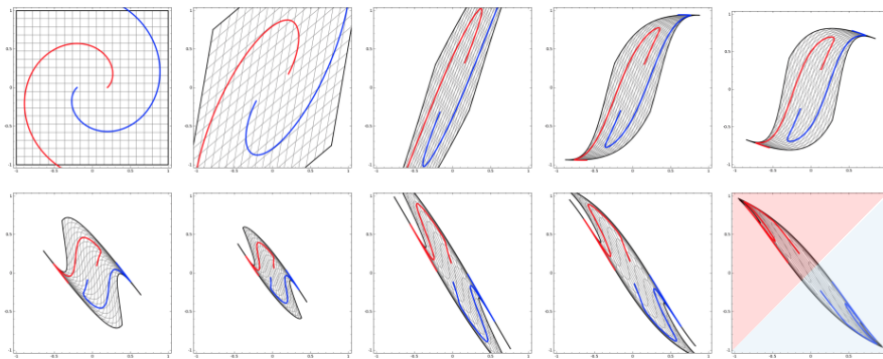
Figure 2: Spiral label data in an original feature space undergoing a sequence of linear and nonlinear transformations into a disentangled representation space.
