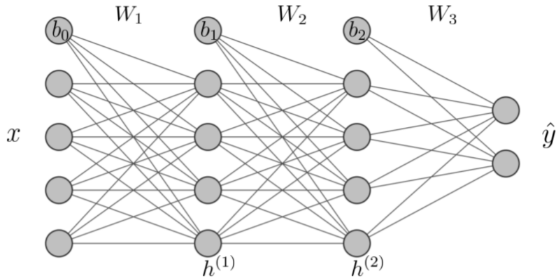
Figure 1: Fully connected artificial neural network diagram
