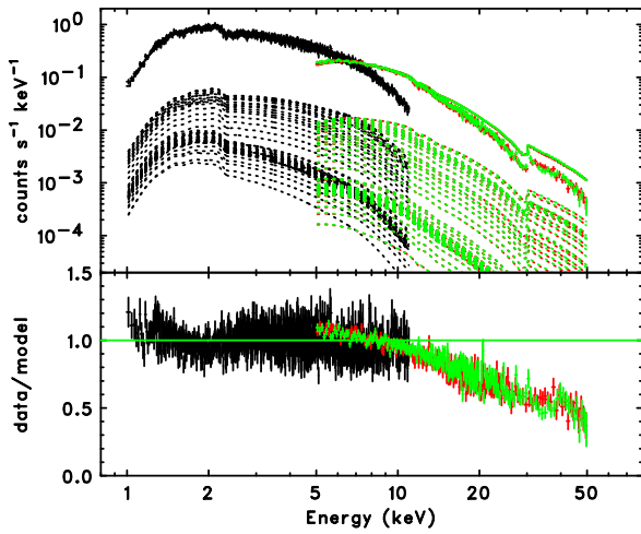
Fig. 3. The SXI (black) and HX1/2 data (red and green) fitted with the composite+PL model accounting for the spatially resolved spectroscopic study of the SNR with Chandra (Guest & Safi-Harb 2018; see also Matheson & Safi-Harb 2005). The individual components contributing to the fitted spectrum are shown as dashed lines. The bottom panel shows the data-to-model ratios and illustrates that this model does not reproduce the spectral shape obtained with the HX1.
