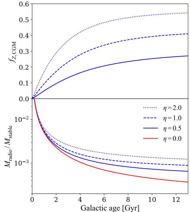
Figure 4. Top panel: Evolution of the fraction of metals, ejected by stars, found outside the galaxy (into the circumgalactic medium, CGM), using the two-infall prescription of Chiappini et al. (1997) for the star formation history (red lines in the top panel of Figure 2). Different lines represent different strength of galactic outflows (see the \eta parameter in Equation 5). Bottom panel: Evolution of the mass ratio between the radioactive and stable isotopes, for different strength of galactic outflows. The adopted yields and half-life are the same as in Figure 2.
