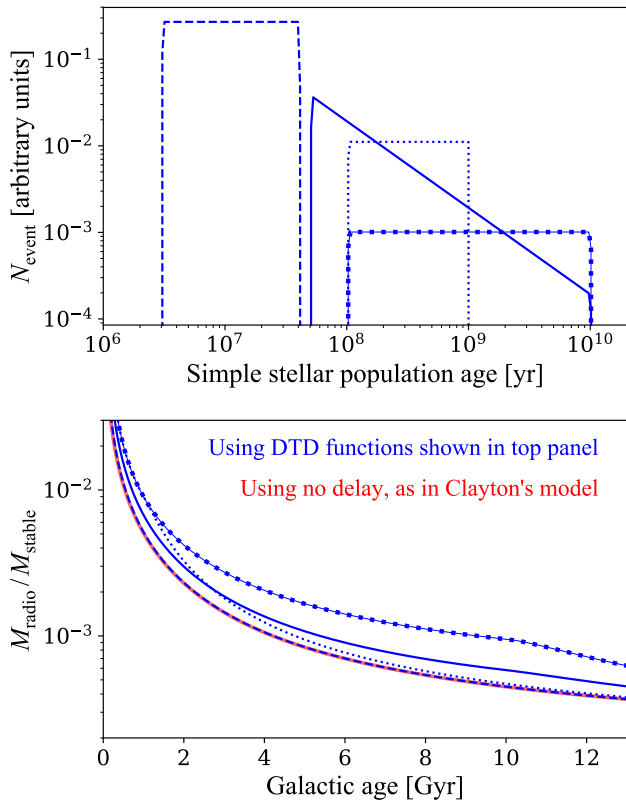
Figure 5. Top panel: Examples of delay-time distribution functions that can be associated with the astronomical events producing the stable and radioactive isotopes. They show how the stellar ejecta are distributed as a function of time in a simple stellar population. Bottom panel: Evolution of the mass ratio between the radioactive and stable isotopes, assuming different delay-time distribution functions. The red line is our fiducial model (red lines in the top panels of Figures 2 and 3), which does not include any delay between the ejection of isotopes and the formation of the progenitor stars, as in Clayton’s model.
