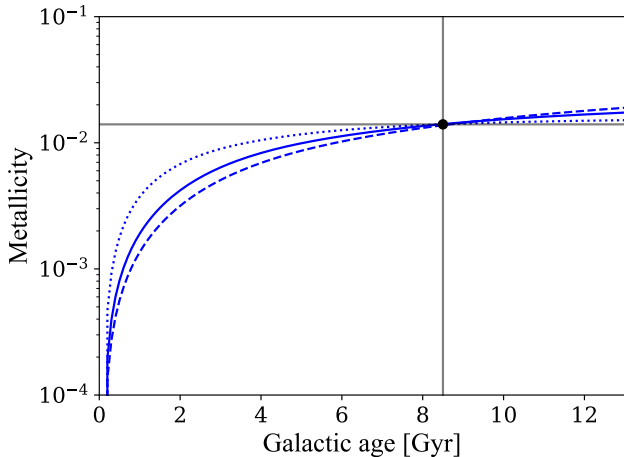
Figure 7. Evolution of the gas metallicity (mass fraction) predicted by the three Milky Way models presented in Figure 6. The vertical and horizontal gray solid lines represent the time at which the Sun is assumed to form, and the Solar metallicity ( Z = 0.014 , Asplund et al. 2009 ), respectively.
