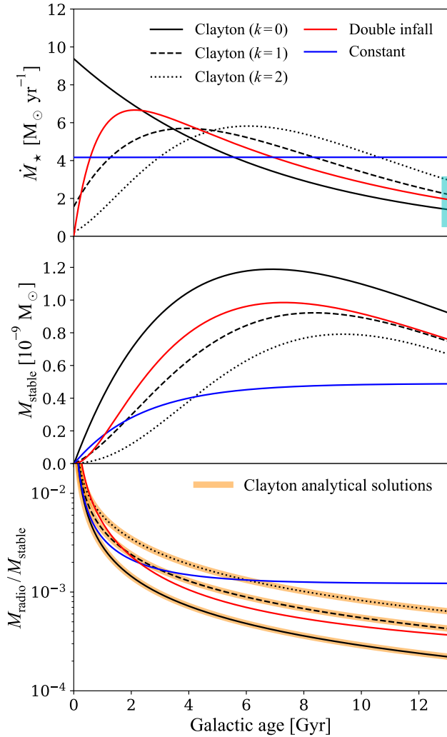
Figure 2. Top panel: Star formation histories calculated assuming different galactic inflow histories: Clayton’s model (black lines), the two-infall prescription of Chiappini et al. (1997) , and a constant inflow history (blue line). The vertical thick cyan line represents the current values derived from observation for the Milky Way ( Robitaille & Whitney 2010 ; Chomiuk & Povich 2011 ). Middle panel: Evolution of the mass of a stable isotope present in the interstellar medium, assuming different star formation histories. Bottom panel: Evolution of the mass ratio between the radioactive and stable isotopes. The thick orange lines represent the analytic solutions of the Clayton’s model. All other lines have been computed using a simplified version of OMEGA+ that mimics the conditions adopted in Clayton’s model (Section 3.1). In all calculations, we assumed a radioactive-to-stable mass ratio of 0.2 for the yields and a half-life of 10 Myr for the radioactive isotopes.
