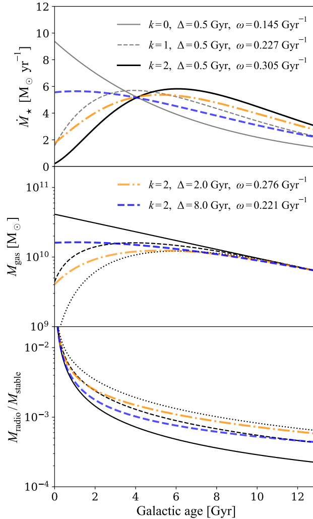
Figure 9. Evolution of the star formation rate (top panel), mass of gas (middle panel), and isotopic mass ratio (lower panel), generated by integrating the system of equations of Clayton (1984, 1988) and by using different input parameters as labelled in the top and middle panels. We refer to Appendix A for a description of the parameters. The cyan bands at 13 Gyr are observational constraints taken from Kubryk et al. (2015).
