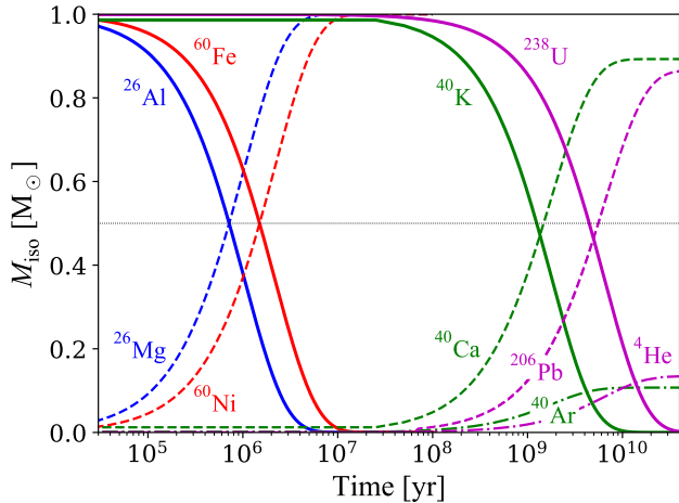
Figure 1. Evolution of the mass of radioactive isotopes (solid lines) along with the rise of their daughter isotopes (dashed and dot-dashed lines), using the decay module included in our chemical evolution codes (Section 2.4). Each color represent a decay process of a specific radionuclide, as indicated on the figure. There is no enrichment process in this figure, and all radioactive isotopes have initially been set to 1 M_{\odot} . The time at which a solid line crosses the thin grey horizontal line represents the half-life of the associated radioactive isotope.
