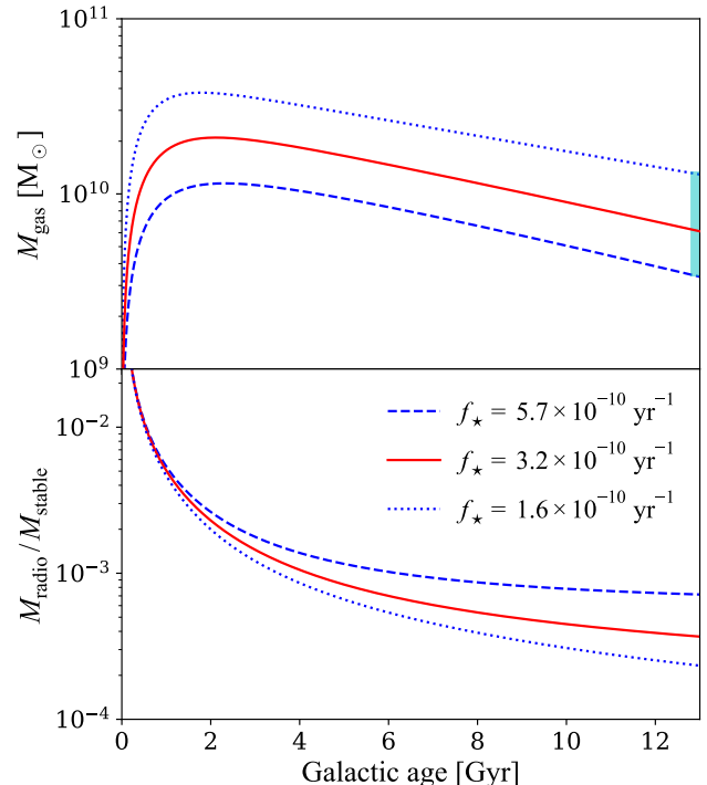
Figure 3. Top panel: Evolution of the mass of gas inside the galaxy, using the two-infall prescription of Chiappini et al. (1997) for the star formation history (red lines in the top panel of Figure 2). Different lines represent different star formation efficiency (see the f_{\star} parameter in Equation 4). The vertical thick cyan line represents the current value derived from observation for the Milky Way (Kubryk et al. 2015). Bottom panel: Evolution of the mass ratio between the radioactive and stable isotopes, for different star formation efficiency.
