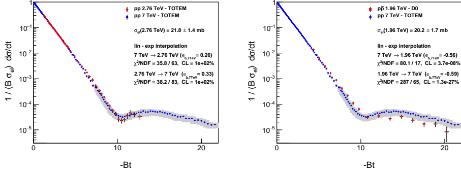
Figure 1. Left panel: For proton-proton elastic scattering, the H(x, s) = \frac{1}{B\sigma_{el}} \frac{d\sigma}{dt} scaling function is energy independent in terms of x = -tB at the TeV energy scale, or specifically, in the \sqrt{s} = 2.76 - 7 TeV energy range. TOTEM preliminary data at \sqrt{s} = 8 TeV [19] also follow this scaling law, while scaling violations are observed at \sqrt{s} = 13 TeV [8]. Right panel: A statistically significant difference is found between the H(x, s) scaling functions for elastic pp collisions at \sqrt{s} = 7.0 TeV and that of p\bar{p} collisions at \sqrt{s} = 1.96 TeV. On both panels, vertical lines stand for the type A (point-to-point fluctuating) errors, while the horizontal lines indicate the point-to-point fluctuating uncertainty of the horizontal errors. Grey vertical bars stand for the type B (point-to-point changing, but overall correlated) errors and the width of this grey bars correspond to the type B errors in the horizontal ( x ) direction. Larger and smaller boxes correspond to two different measurements at \sqrt{s} = 7 TeV, detailed in Refs. [20, 21], respectively.
