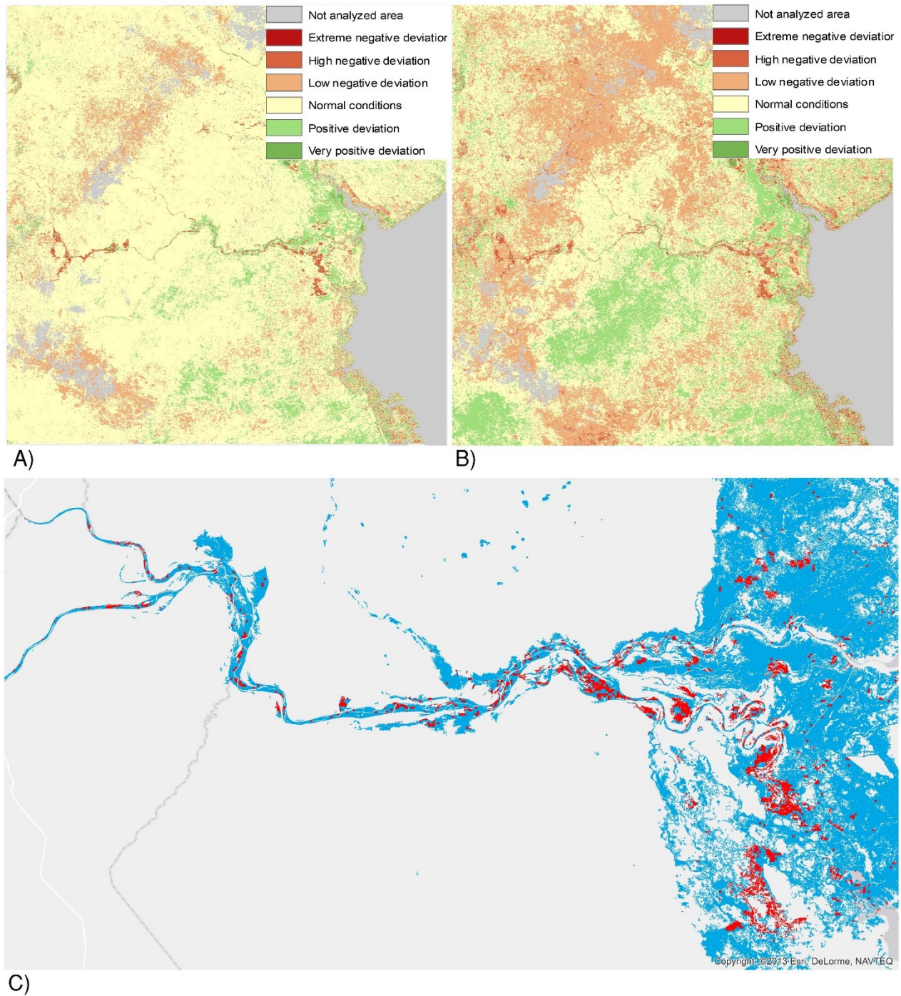
Figure 10. An example of anomaly maps of SMI (A) and LOS (B) computed with reference to the MOD13Q1 dataset for the 2018-2019 growing season, which was affected by the Cyclone Idai. Maps show the spatial distribution of percent deviations of selected phenological metric from to the historical average value (estimated from the 2000-2018 time-series). These maps, produced in near real-time or immediately after the examined growing season, can support the identification of critical areas where major damages to vegetation productivity are expected. Similar maps can be generated with reference to other significant PM for monitoring purposes and vegetation restoration evaluation. For the purpose of the examined case study, vegetated patches falling in the flooded areas (in blue in C) showing extreme negative LOS deviations were mapped (in red in C).
