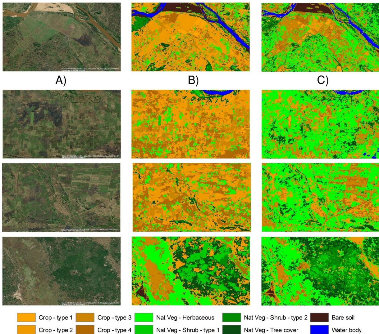
Figure 3. Examples of land cover maps obtained through unsupervised classification based on: b) NDVI monthly profile (August 2017 - November 2018) derived from Sentinel-2 imagery; c) VIS+NIR spectral signature extracted from Sentinel-2 multispectral monthly composite (July 2018). A high spatial resolution WorldView-3 image (DigitalGlobe Vivid mosaic; acquisition date 8/2/2018) is also reported for reference purposes (a). A K-Means Iterative Minimum Distance algorithm has been adopted, considering the following parameters: number of classes = 12; maximum number of iterations = 100 with change threshold value = 1%; standard deviation to use around the class mean = 0.05. Reported examples show that VI temporal profile-based classification better mapped crops, especially in those areas with high levels of land fragmentation and mixture of cultivated and natural vegetation classes. In fact, some crop types and natural vegetation classes (mainly herbaceous) present a low spectral separability if tested in a single monthly image (July, in this study).
