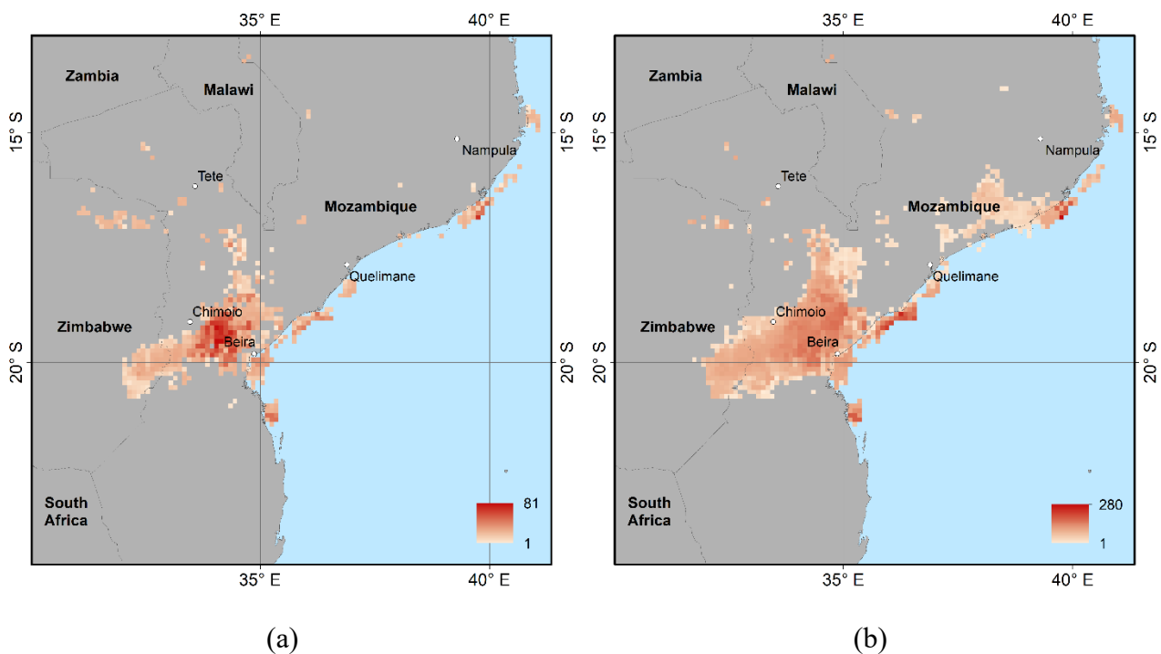
Figure 4. Number of alerts provided by ERDS during the period between 5 and 24 March 2019 using GPM data as input and aggregation intervals equal to 12 hours (a) and 48 hours (b). Most of the alerts were issued in the area near Beira, where the combination of heavy rainfall and river overflow created an “inland ocean”.
