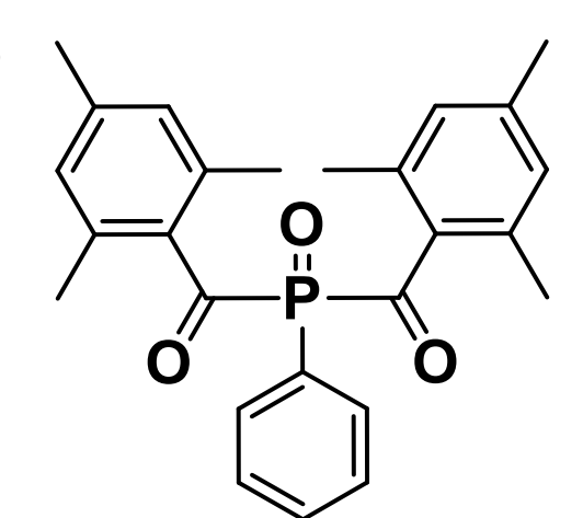
Phenylbis(2,4,6-trimethylbenzoyl)phosphine oxide
