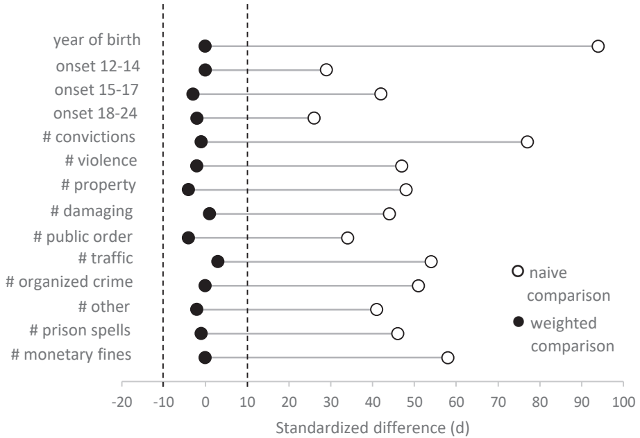
Figure 3. Standardized differences of pretreatment covariates before and after applying matching weights
