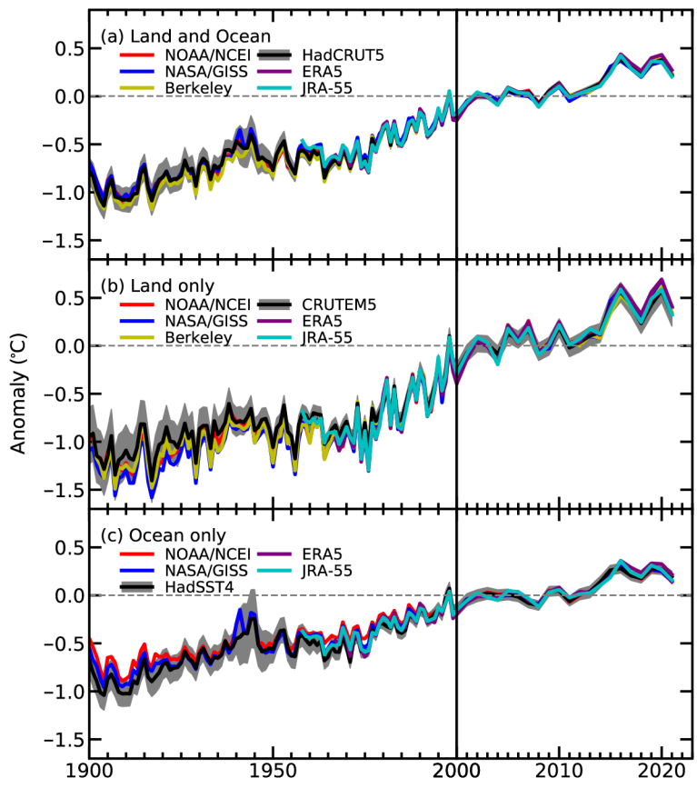
Fig. 2.1. Global average surface air temperature anomalies (°C; 1991–2020 base period). In situ estimates are shown for NOAA/NCEI (Zhang et al. 2019), NASA-GISS (Lenssen et al. 2019), Berkeley Earth (Rhode and Hausfather 2020), HadCRUT5 (Morice et al. 2021), CRUTEM5 (Osborn et al. 2021), and HadSST4 (Kennedy et al. 2019). Reanalysis estimates are shown from ERA5 (Hersbach et al. 2020), including from the preliminary ERA5 back-extension (Bell et al. 2021) for 1967–2021, and JRA-55 (Kobayashi et al. 2015). Please note change in x-axis scale pre/post 2000.
