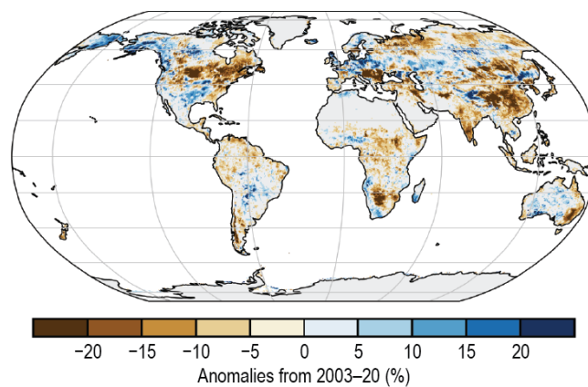
(ae) Fraction of Absorbed Photosynthetically Active Radiation
