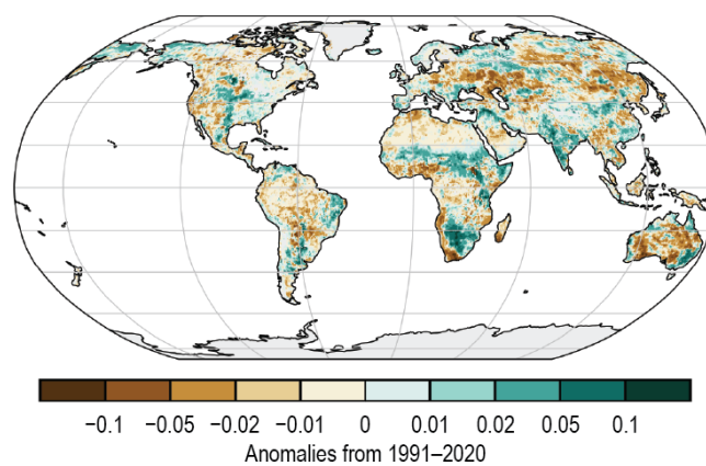
(ag) Vegetation Optical Depth
