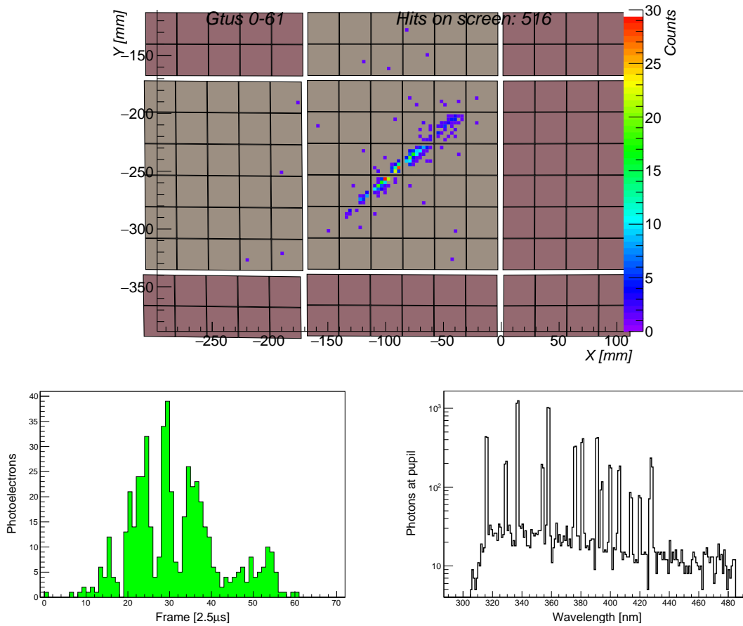
Figure 10: Distribution of photoelectrons from an EAS generated by a 100 EeV proton arriving at the zenith angle of 60^\circ simulated with ESAF. Only signal from the shower is shown. Top: distribution of the signal on the focal surface. Bottom left: the corresponding time distribution of photoelectrons. Bottom right: the spectrum of photons at the detector entrance.
