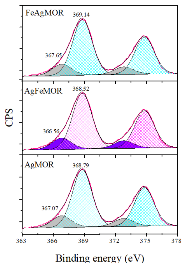
Figure 4. Ag 3d_{5/2} photoelectron spectra of the studied samples.
