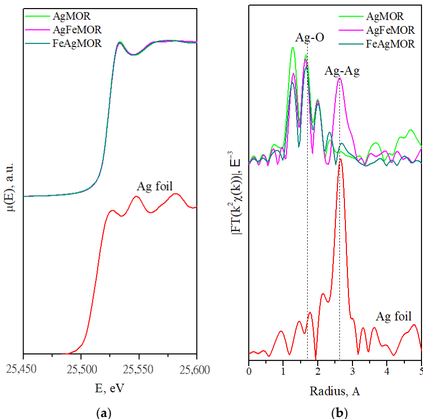
Figure 5. (a) Ag K-edge XANES spectra; (b) Ag K-edge EXAFS Fourier transforms taken in the k-range from 3 to 15 Å -1 .
