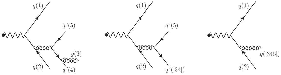
Figure 1. Sample Feynman diagrams for three-jet production in leptonic collisions: NNLO double real emission (left), NLO single real emission (middle), Born process (right).
