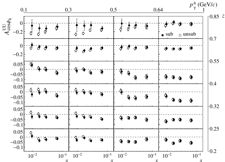
Figure 6: Same as Fig. 5 for negative hadrons.
