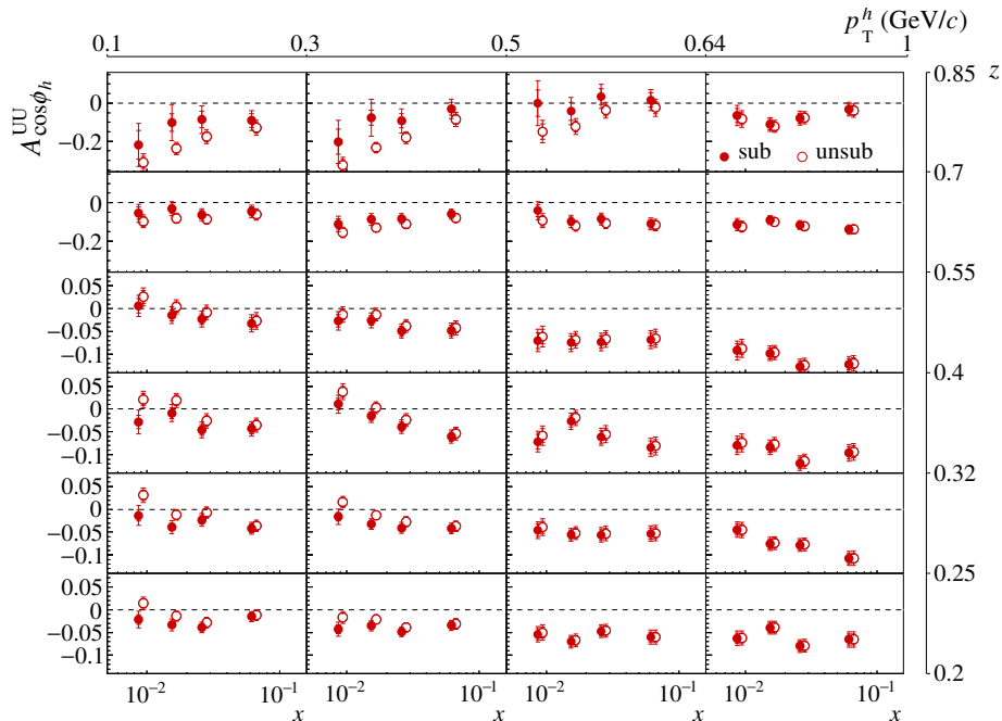
Figure 5: A_{\cos\phi_h}^{UU} asymmetry on ^6\text{LiD} for h^+ after subtracting from the asymmetry published in Ref. [3] the contribution of exclusive-VM hadrons, as function of x , in z and p_T^h bins (closed circles). Inner (outer) error bars denote statistical (total) uncertainties. The open circles show the unsubtracted asymmetry.
