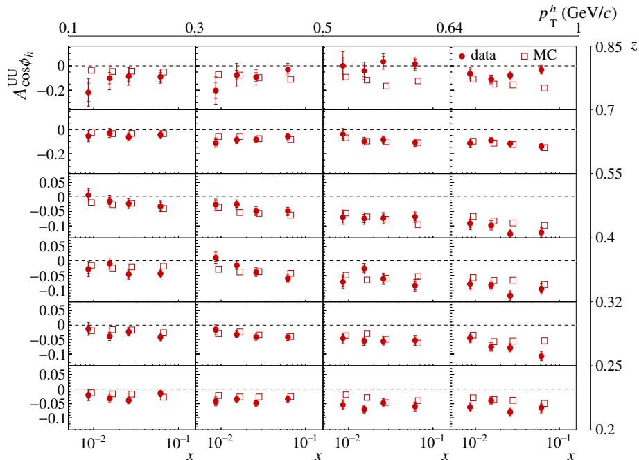
Figure 9: Comparison between the A_{\cos\phi_h}^{UU} asymmetry, as function of x , in z and p_T^h bins, for h^+ on ^6\text{LiD} after subtracting the exclusive-VM hadron contribution (closed circles) and the results of a Monte Carlo simulation (open squares) which includes the Cahn effect.
