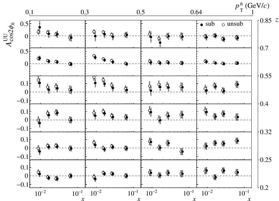
Figure 8: Same as Fig. 7 for negative hadrons.
