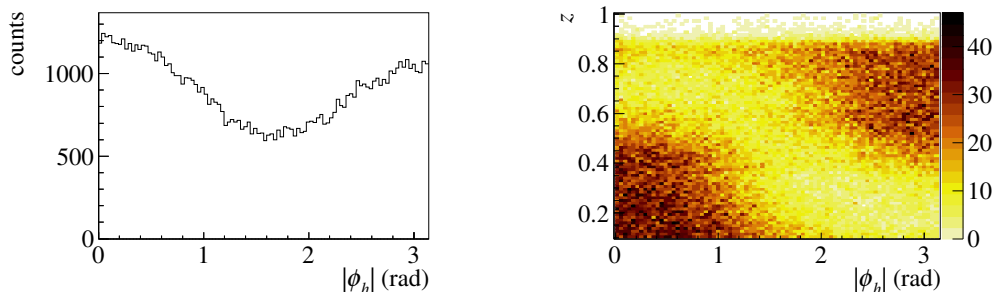
Figure 2: Distribution of |\phi_h| (left panel) and correlation between z and |\phi_h| (right panel) for positive exclusive-VM hadrons.
