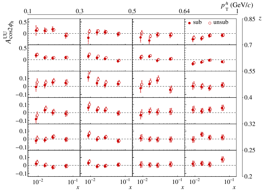
Figure 7: A_{\cos 2\phi_h}^{UU} asymmetry on {}^6\text{LiD} for h^+ after subtracting from the asymmetry published in Ref. [3] the contribution of exclusive-VM hadrons, as function of x , in z and p_T^h bins (closed circles). Inner (outer) error bars denote statistical (total) uncertainties. The open circles show the unsubtracted asymmetry.
