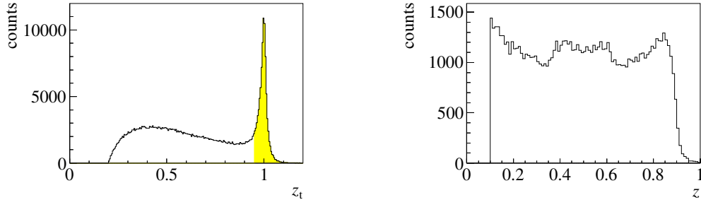
Figure 1: Left panel: distribution of z_t for the events with only two reconstructed hadrons with opposite charge. The exclusive events are selected by the cut z_t > 0.95 . Right panel: z distribution for the positive hadron of the selected pairs.
