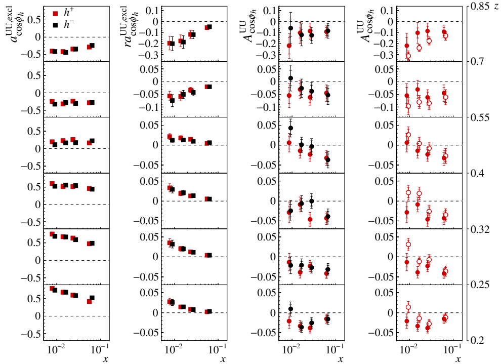
Figure 3: First column: a_{\cos \phi_h}^{UU,excl} amplitude for h^+ (red squares) and h^- (black squares). Second column: r a_{\cos \phi_h}^{UU,excl} for h^+ (red squares) and h^- (black squares). Third column: A_{\cos \phi_h}^{UU} asymmetry after the subtraction of exclusive-VM hadron contribution for h^+ (red circles) and h^- (black circles). Last column: comparison between the asymmetry for h^+ before (open circles) and after (full circles) exclusive-VM hadron subtraction. From bottom to top, results for increasing values of z are shown, as indicated on the very right of the figure. All the results refer to the first p_T^h bin ( 0.1 \text{ GeV}/c < p_T^h < 0.3 \text{ GeV}/c ).
