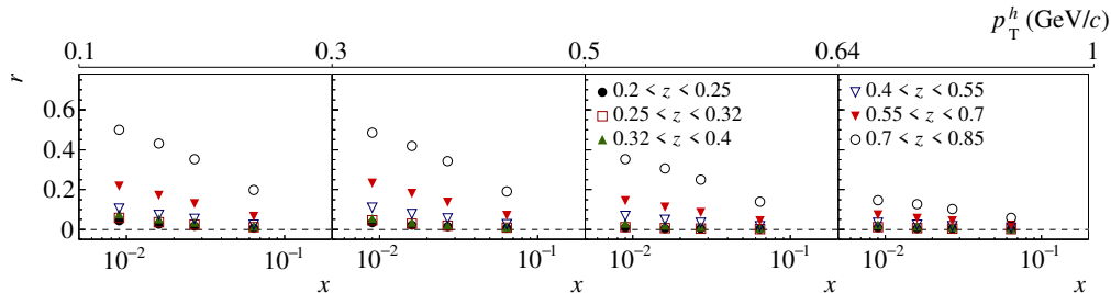
Figure 4: Fraction r of exclusive-VM hadrons evaluated as function of x in the different z and p_T^h bins.
