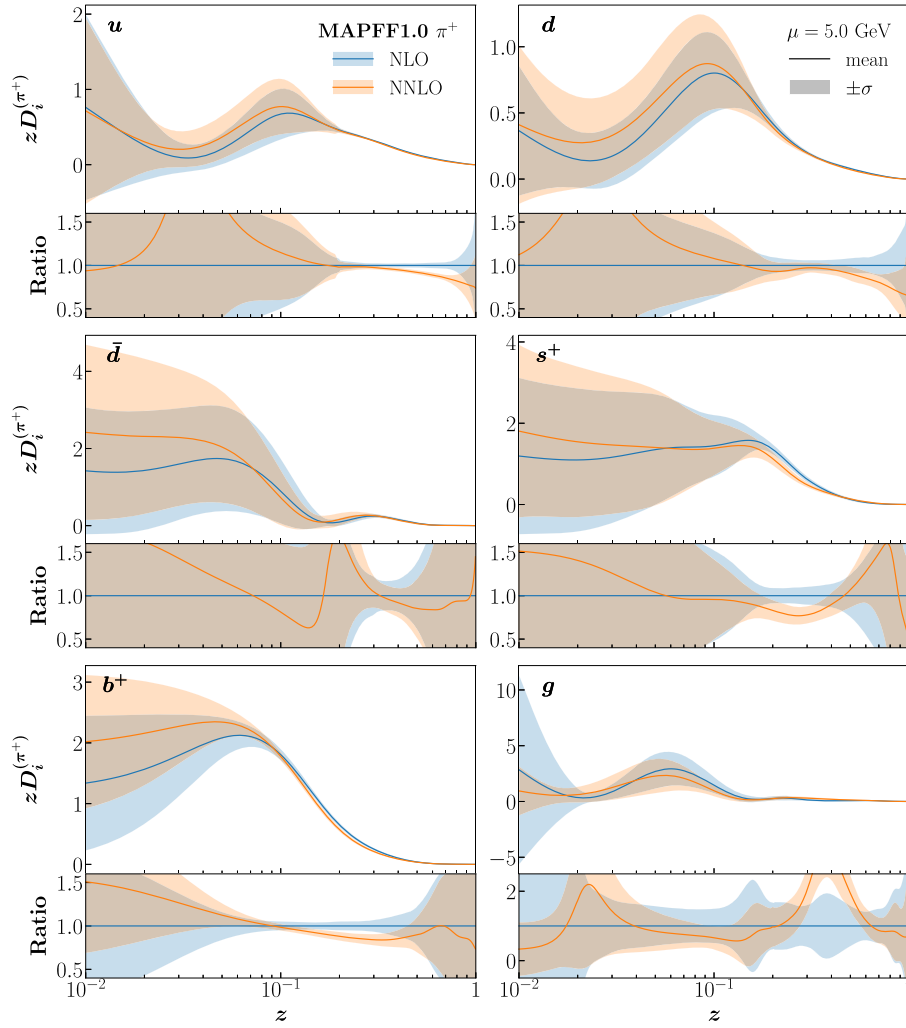
Fig. 1. Comparison of the NLO and NNLO FFs for positively charged pions. We display the D_u^{\pi^+} , D_d^{\pi^+} , D_{\bar{d}}^{\pi^+} , D_{s^+}^{\pi^+} , D_{b^+}^{\pi^+} and D_g^{\pi^+} FFs at \mu = 5 GeV. Expectation values and uncertainties correspond to the mean and standard deviation computed over the ensemble of FF replicas. For each FF we plot the absolute distributions in the upper panels and their ratio to the central value of the NLO FFs in the lower ones.
