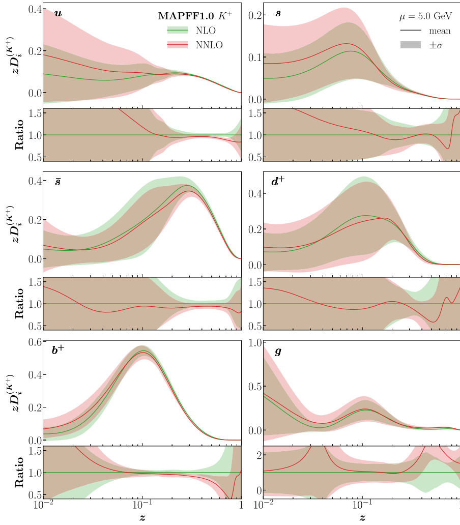
Fig. 2. Same as Fig. 1 for kaons, now displaying D_u^{K^+} , D_s^{K^+} , D_{\bar{s}}^{K^+} , D_{d^+}^{K^+} , D_{b^+}^{K^+} and D_g^{K^+} .
