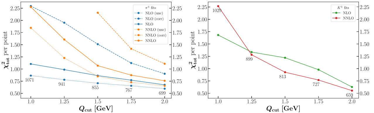
Fig. 3. The value of the total \chi^2 per data point as a function of the cut on Q , Q_{\text{cut}} , applied to the SIDIS data in the pion (left) and kaon (right) FF fits. For each value of Q_{\text{cut}} , the number of data points included in the fits are also displayed. Both NLO and NNLO fits, are considered. In the case of the fit of pion FFs, various correlation models for the COMPASS data are taken into account, see the text for details.
