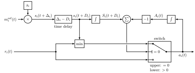
Figure 5: Block-diagram of the proposed admission controller. It uses feedback from the queue-size (computed using feedback from m_i^{\text{ref}}(t) and a_i(t) ) in order to compute whether the incoming packets can be admitted or not. As shown in Theorem 3.2 the feedback-law (or admission policy) derived here is able to admit as many packets as possible, while still guaranteeing that all the admitted packets will meet the node deadline D_i . It should be noted that it is assumed that \Delta_i > D_i .
