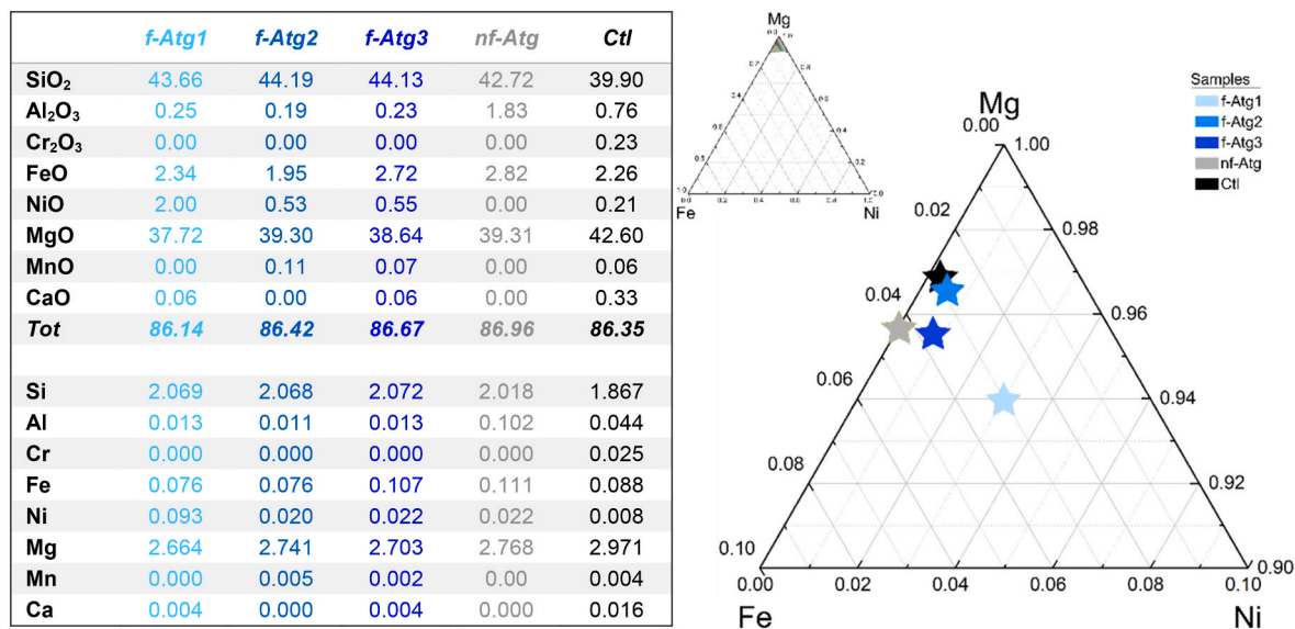
Fig. 1. Chemical composition of the Atg specimens. Representative chemical analyses (in weight percent of oxides) and structural formulae (in atoms per formula unit) of Atg and Ctl (left). Chemical analyses were normalized on the basis of seven oxygen. The full set of EDS analyses is reported in (Petriglieri et al., 2021). Ternary diagram (right) considering Mg, Fe, and Ni elements showing the variability in chemical composition of antigorite samples and Ctl. Specimen f-Atg1 exhibits a high Ni content and a relative low Mg + Fe content. Data were plotted as atoms per formula unit.
