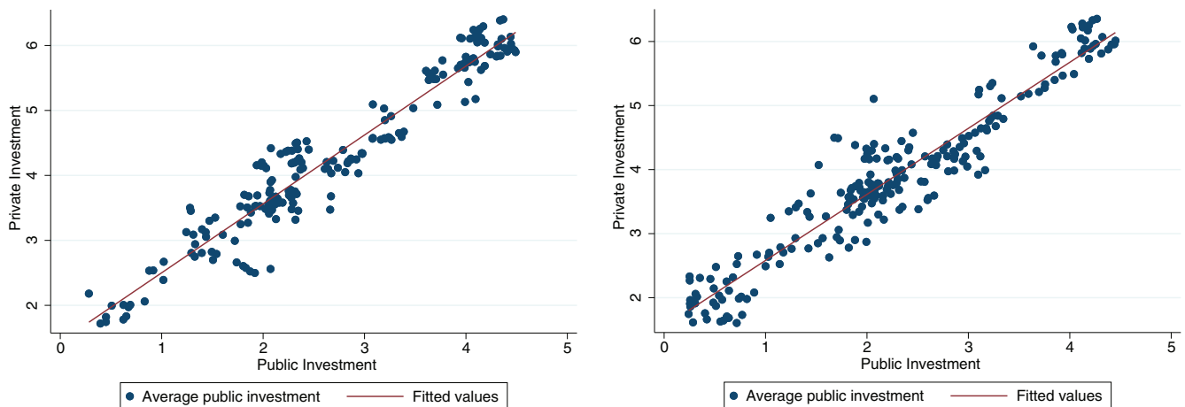
FIGURE 3 (a) Correlation between the log of private and of public investment for a growth rate of GDP <2%. (b) Correlation between the log of private and of public investment for a growth rate of GDP \geq 2\% . Source: Ameco database [Colour figure can be viewed at wileyonlinelibrary.com ]
