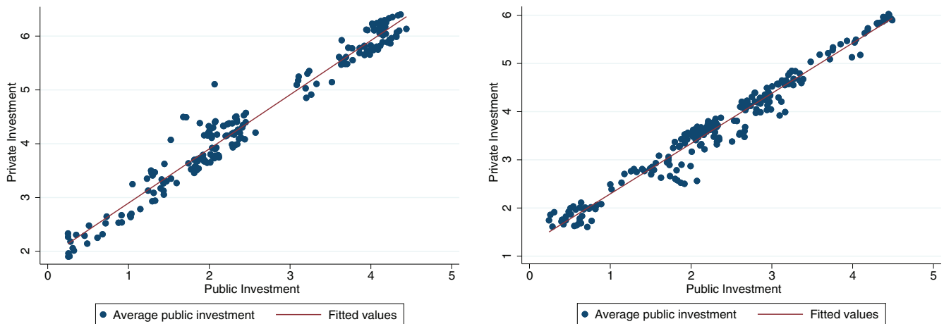
FIGURE 2 (a) Correlation between the log of private and of public investment for a ratio of public to private investment <0.2. (b) Correlation between the log of private and of public investment for high levels of a ratio of public to private investment \geq 0.2 . Source: Ameco database [Colour figure can be viewed at wileyonlinelibrary.com ]
