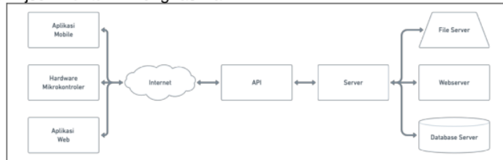
Gambar 9. Blok Diagram Aplication Program Interface
