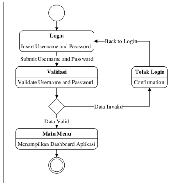
Gambar 5. Statechart Proses Login
