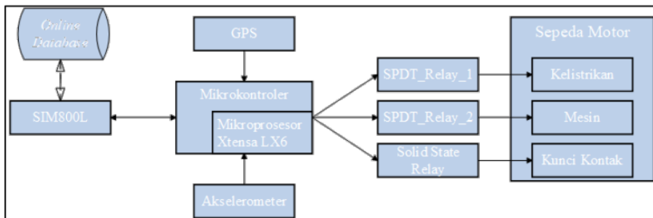
Gambar 3. Blok Diagram Hardware
