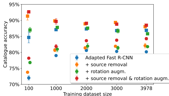
Fig. 6. Ablation study of source removal and rotation augmentation for the large and bright source component training datasets of increasing size. Round (squared) markers show performance on the full validation (partial training) dataset. Data points and their error bars are the mean and standard deviation of three training runs with different random seeds and otherwise equal setup. The horizontal scatter of the data points around each x-axis tick mark is artificially created to prevent overlap.
