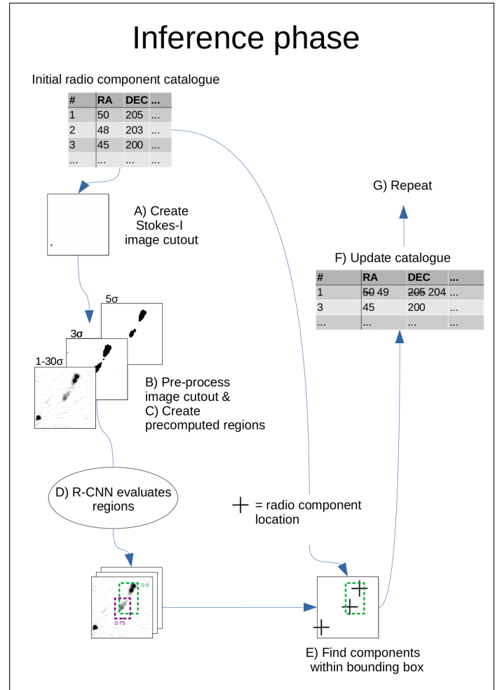
Fig. 3. Diagram of inference phase. We start from a radio component catalogue created by PyBDSF . A) We create an image cutout centred on a radio component from the initial catalogue. B) We pre-process the image for the R-CNN. C) We pre-compute regions (see Section 4.4). D) The R-CNN predicts several regions and corresponding prediction scores based on the image (known as a ‘forward pass’). E) We select the region that covers the central radio component and has the highest prediction score. We then look for the radio component coordinates that lie within this region. F) These radio components will enter the updated radio source catalogue combined into a single entry. G) Steps A-E are repeated for all radio components in our inference dataset.
