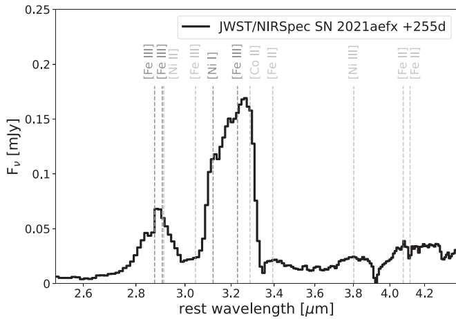
Figure 5. JWST/NIRSpec line identifications in the 3\ \mu\text{m} region, previously unobserved for SN Ia. The main line features arise from [Fe III] 2.874\ \mu\text{m} and 2.905\ \mu\text{m} , and [Ni I] 3.120\ \mu\text{m} and [Fe III] 3.229\ \mu\text{m} emission (gray). Several possible weaker lines that may be blended with the dominant lines are shown in light gray. Details of the dominant lines can be found in Table 2.
