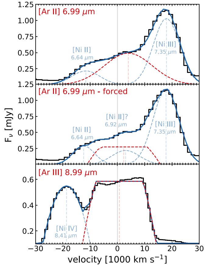
Figure 11. Observed argon emission-line profiles for SN 2021aefx at +255 days (black) compared to model line emission from a Gaussian emission distribution for [Ar II] 6.985 \mu\text{m} (top); a thick uniform shell or hollow uniform sphere emission distribution for [Ar III] 8.991 \mu\text{m} with an inner radius corresponding to v_{\text{min}} = 8700 \pm 200 \text{ km s}^{-1} , and an outer radius corresponding to v_{\text{max}} = 13,500 \pm 300 \text{ km s}^{-1} (bottom); and a thick shell distribution for [Ar II] 6.985 \mu\text{m} , which has been forced to have the same inner and outer radius as the [Ar III] fit (middle). The model profile for the central line is shown in dotted red, with contributions from other lines shown in dotted blue and the full modeled superposition of lines shown in solid blue.
