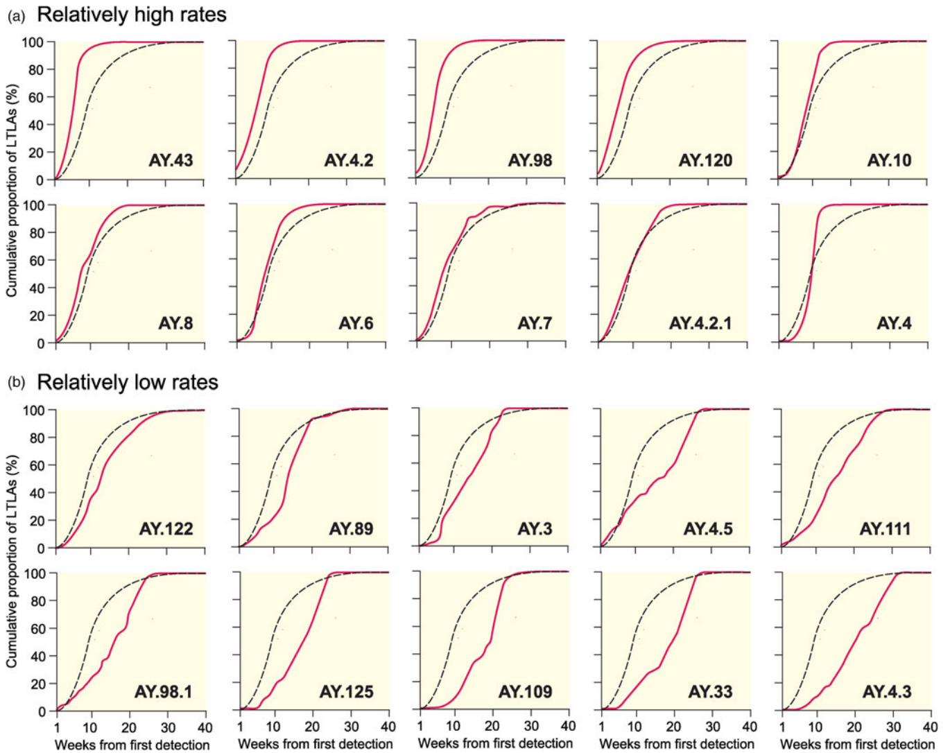
Fig. 6. Spatial growth curves for sample Delta sublineages in England, March–December 2021. Curves have been formed in the manner of the lower graphs in Figure 2, with the average curve plotted for reference. Lineages are ordered according to the values of \bar{t}_{LE} in Table 1 and are defined as having relatively high (i.e. low values of \bar{t}_{LE} ; upper graphs, a) and relatively low (i.e. high values of \bar{t}_{LE} ; lower graphs, b) rates of spatial growth.
