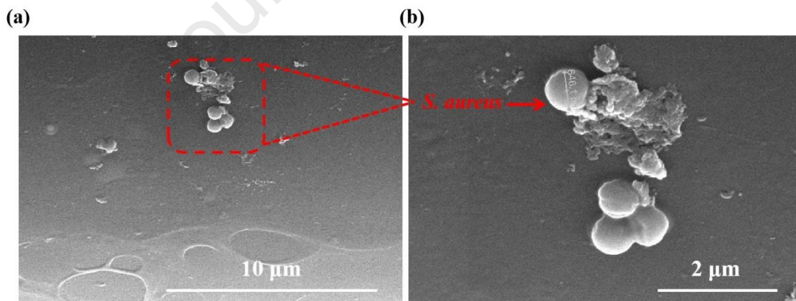
Fig. 4: SEM images of the functional SCS-based EDFL biosensor bound with S. aureus with different scale bar: (a) 10, and (b) 2 µm.
