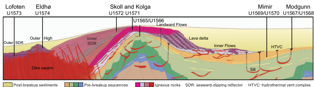
Figure F2. Schematic transect across a volcanic passive margin indicating the relative position of the volcanic seismic facies units and Expedition 396 site locations.
