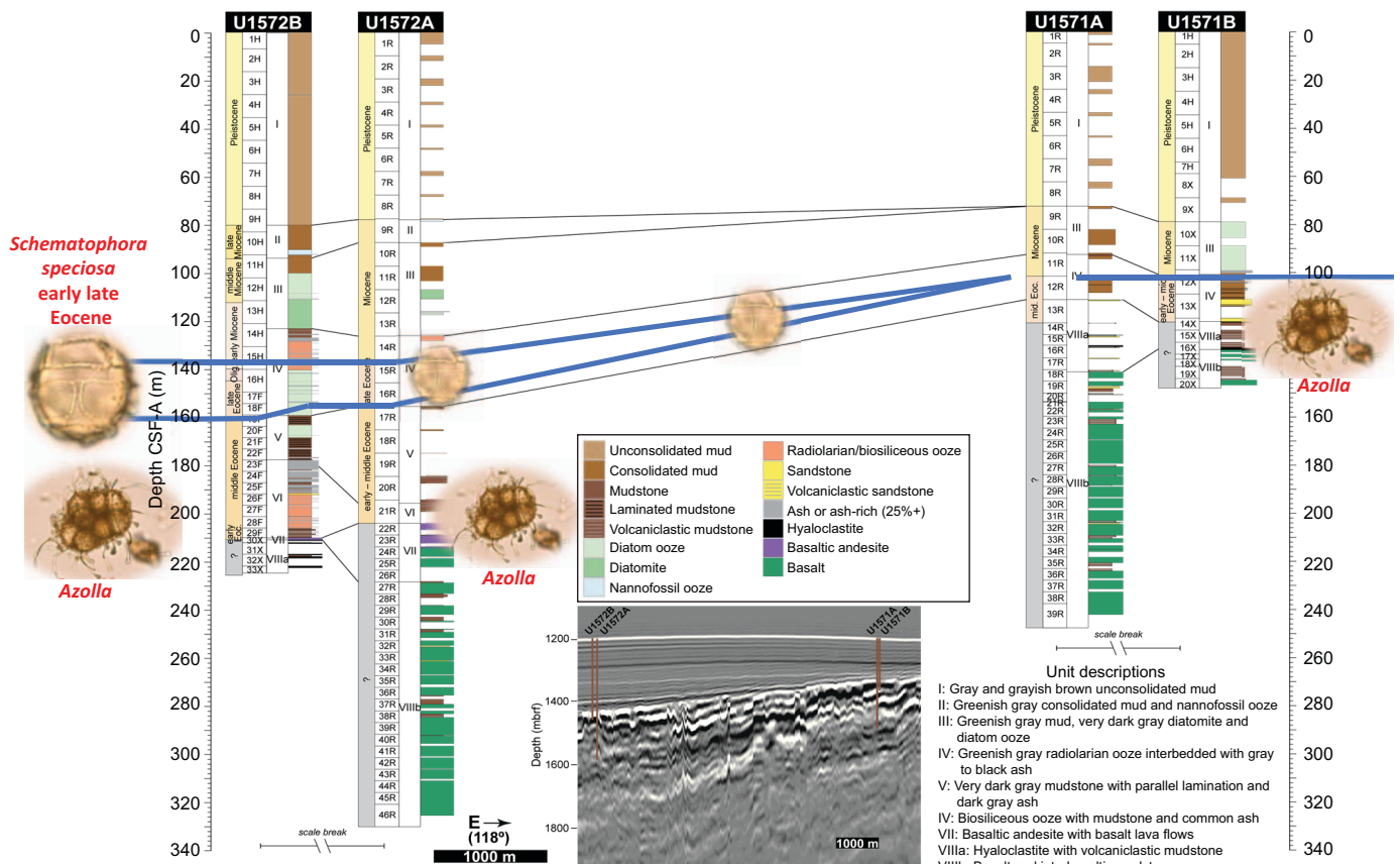
Figure F17. Lithostratigraphic and chronostratigraphic correlation panel, Sites U1571 and U1572. Note the absence of the upper Eocene section at Site U1571. ? = unknown age.
