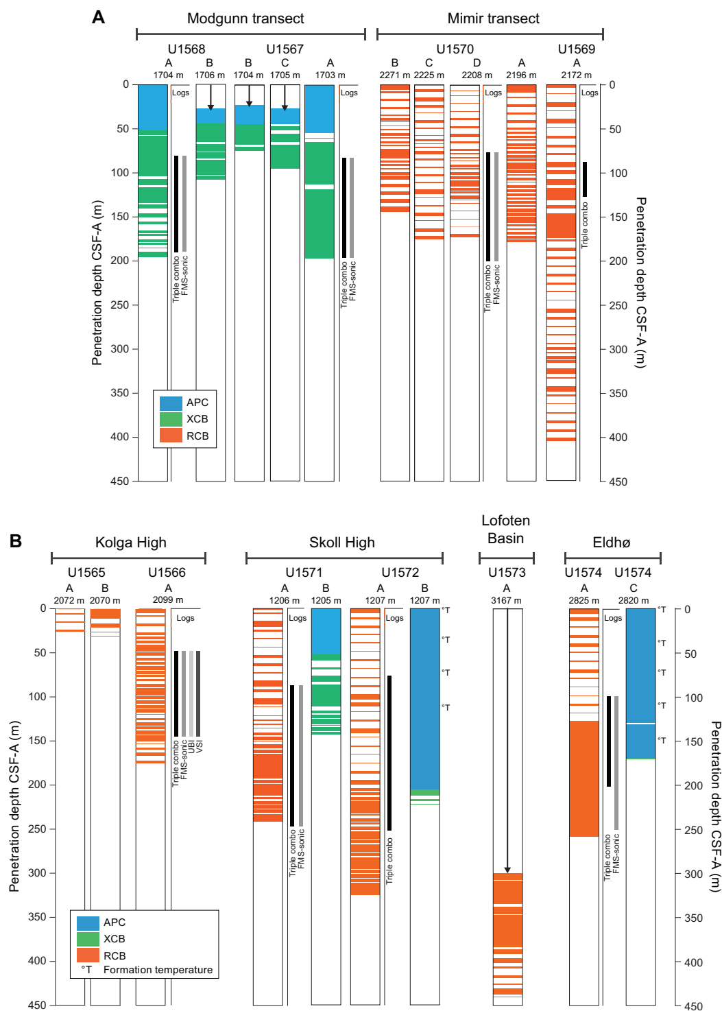
Figure F4. Expedition 396 sites, recovery, and downhole measurements. A. Transects that addressed PETM causes and evolution at Modgunn Arch and Mimir High. B. Transects that addressed igneous basement objectives, including sampling of the subbasalt geology at Kolga High, the Inner SDR units at Skoll High, the Outer High at Eldhø, and the Outer SDR in the Lofoten Basin. FMS = Formation MicroScanner, APC = advanced piston corer, XCB = extended core barrel, RCB = rotary core barrel, UBI = Ultrasonic Borehole Imager, VSI = Versatile Seismic Imager.
