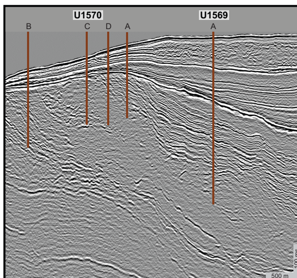
Figure F6. Arbitrary high-resolution 3-D seismic line along the Mimir Transect on the Vøring transform margin showing the relative location of Site U1569 and U1570 boreholes.
