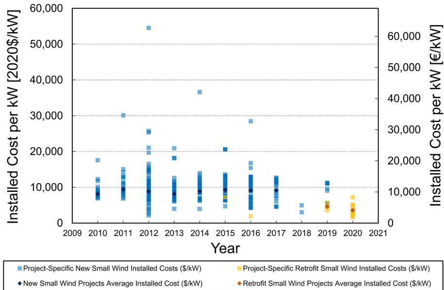
Figure 6. Installed cost per kilowatt for newly installed or retrofit projects in the United States (Orrell et al., 2021).
