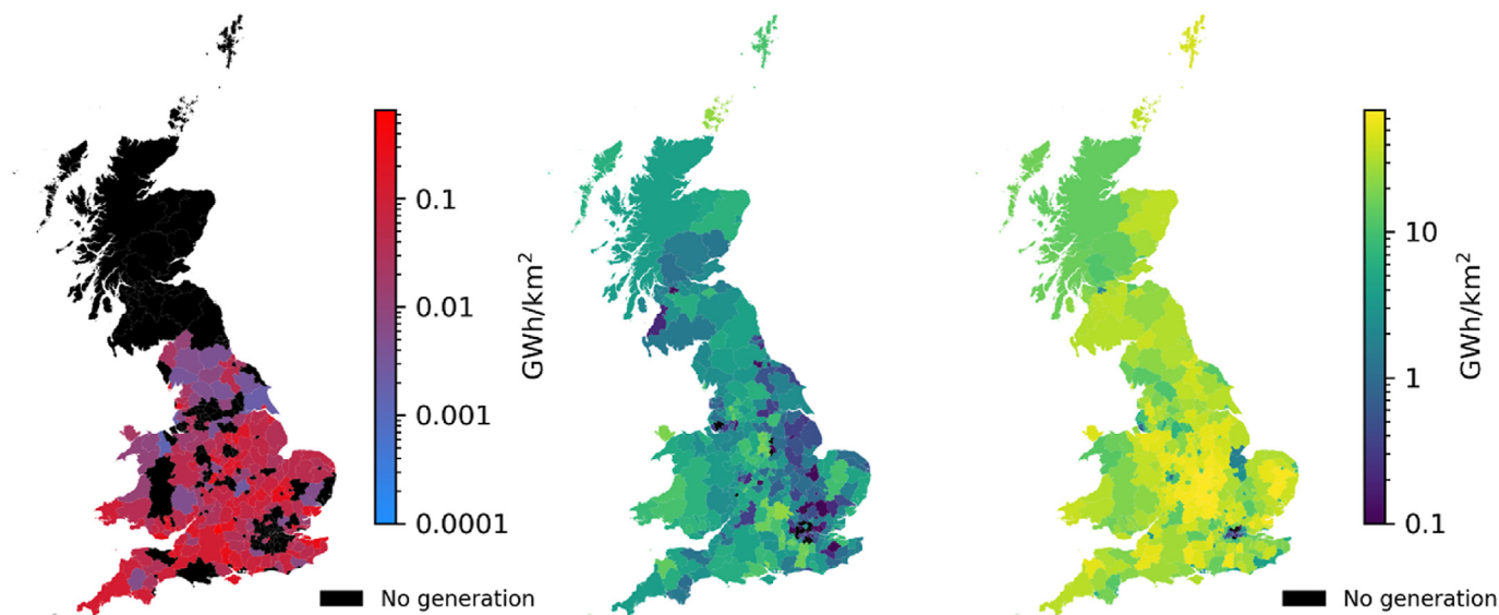
Fig. 4. Ground-mounted solar PV: generation in 2018 (left, [25,26]), technical potential in high restriction scenario (middle) and low restriction scenario (right) respectively, in units of GWh/km 2 . The data is normalised by the total area of each LA and plotted on two separate logarithmic axes.
