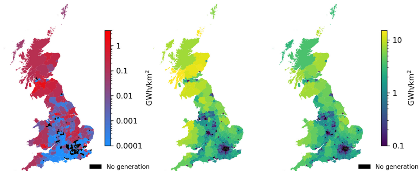
Fig. 3. Onshore wind: generation in 2018 (left, [25,26]), technical potential (middle) and potential at scenicness \leq 5.8 (i.e. the 75% quartile, right), in units of GWh/km 2 . The data is normalised by the total area of each LA and plotted on two separate logarithmic axes.
